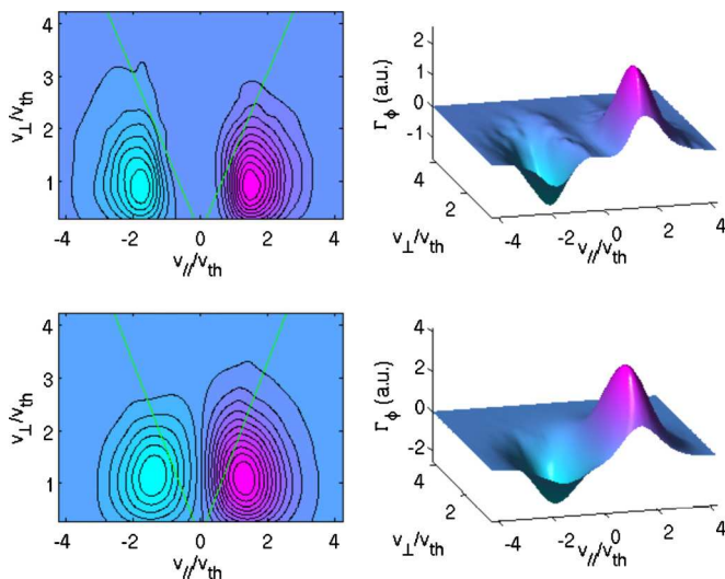
FIG. 19. (Color online) Phase space structures of momentum flux in \nabla T_e -driven (top) and \nabla n -driven (bottom) CTEM turbulence.
