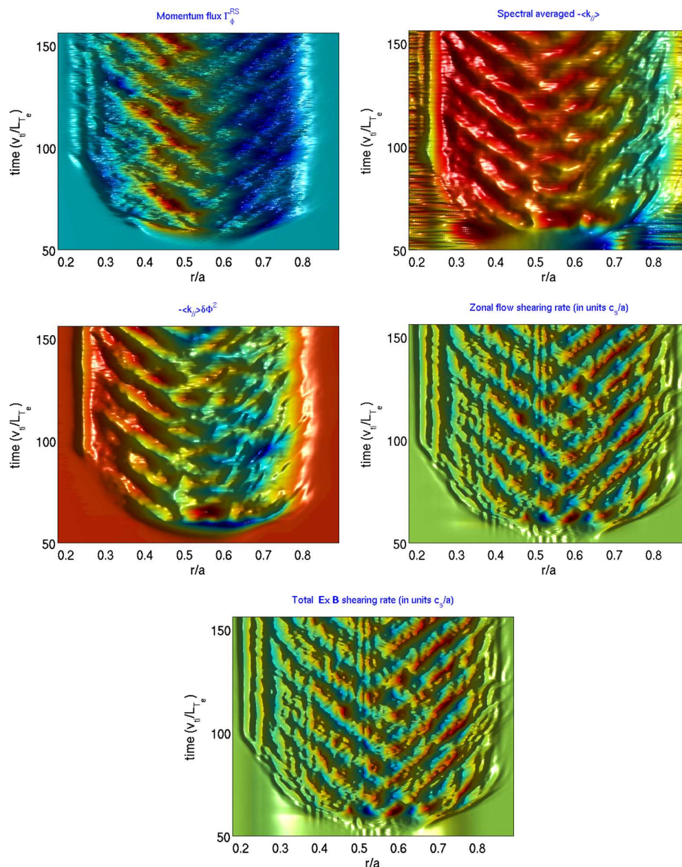
FIG. 13. (Color online) Spatiotemporal evolution of radial flux of toroidal momentum (top-left), \langle k_{\parallel} \rangle \Sigma \delta\Phi_{mn}^2 (midleft), spectrum-averaged \langle k_{\parallel} \rangle (top-right), zonal flow shearing rate (midright), and total \mathbf{E} \times \mathbf{B} shearing rate (bottom) from simulation of CTEM turbulence.
