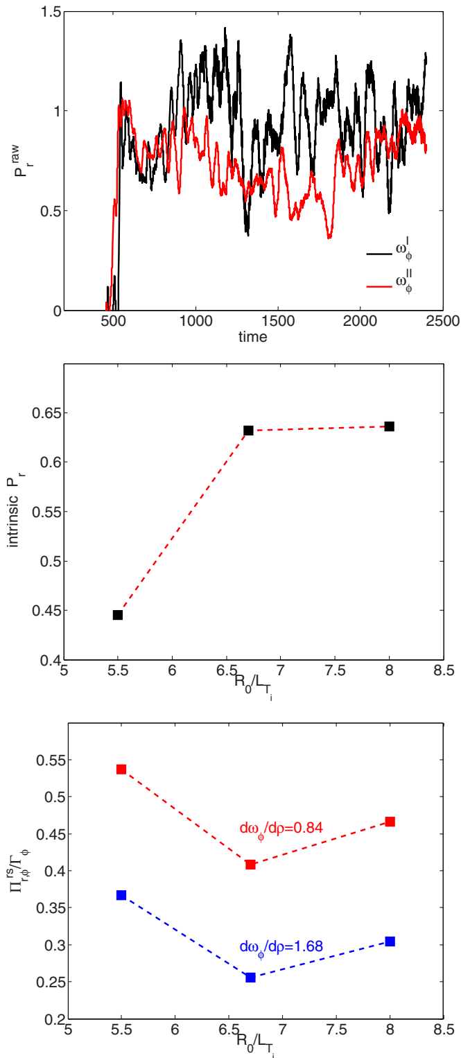
FIG. 6. (Color online) Time (normalized by L_T/v_{th} ) evolution of raw Prandtl number from two simulation with R_0/L_{Ti}=5.5 and different rotation gradients (top), intrinsic Prandtl number vs R_0/L_{Ti} (middle), and ratio of residual stress over total momentum flux vs rotation gradient and R_0/L_{Ti} (bottom).
