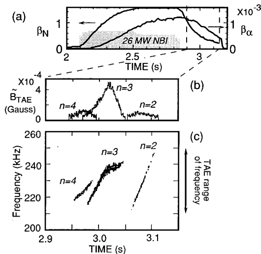
FIG. 7. The alpha-driven TAE mode in TFTR occurring \approx 0.1 s after neutral beam injection in a D-T discharge with weak central magnetic shear. (a) The evolution of \beta_N and \beta_\alpha . (b) The occurrence of magnetic fluctuations with different toroidal mode numbers is observed. (c) The evolution of the frequency of the magnetic fluctuations is consistent with the density-dependent TAE frequency, and mode timing is in reasonable agreement with the theoretical prediction. 77
