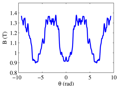
FIG. 2. (Color online) Standard B vs. \theta grid for QAS3-C82, with s = 0.875 , \alpha = \pi/3 , and \theta_0 = 0 .
