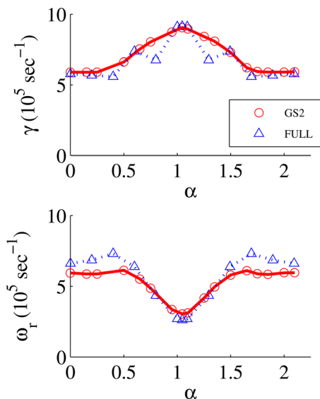
FIG. 5. (Color online) Variation of \gamma and \omega_r with \alpha at constant s=0.875 and \theta_0=0 with \eta_i = \eta_e = 3 and k_y \rho_i (\alpha = \frac{\pi}{3}) = 0.3983 .
