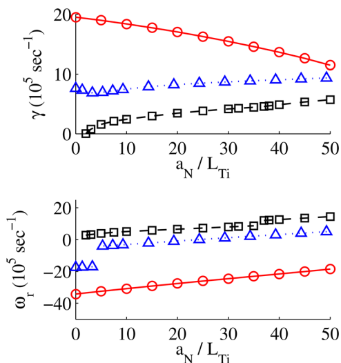
FIG. 13. (Color online) Variation from GS2 of \gamma and \omega_r with a_N/L_{Ti} with k_y\rho_i = 0.3983 . Circles: a_N/L_n = 52.4 , a_N/L_{Te} = 0.0 ; triangles: a_N/L_n = 13.1 , a_N/L_{Te} = 39.3 ; and squares: a_N/L_n = 0.0 , a_N/L_{Te} = 0.0 .
