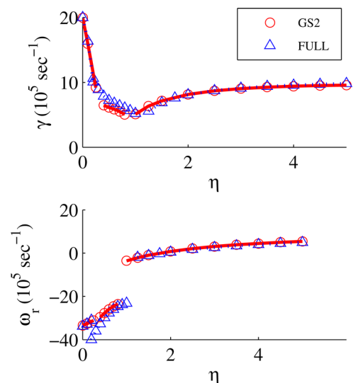
FIG. 7. (Color online) Variation of \gamma and \omega_r with \eta_i = \eta_e with k_y \rho_i = 0.3983 .
