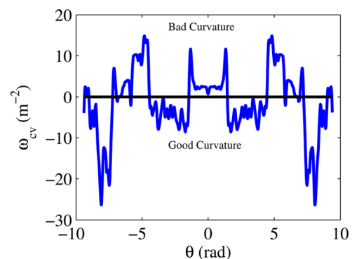
FIG. 4. (Color online) Variation of the curvature drift frequency ( \omega_{cv} = (\mathbf{k}_{\perp}/n) \cdot \mathbf{b} \times [\mathbf{b} \cdot \nabla \mathbf{b}] ) (for n = 1 ) along \theta for QAS3-C82, with s = 0.875 , \alpha = \pi/3 , and \theta_0 = 0 .
