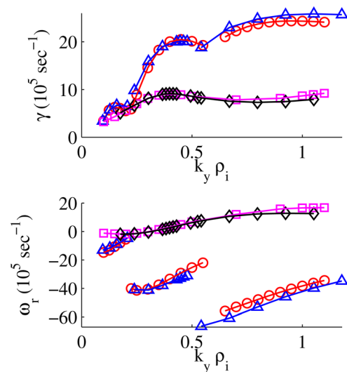
FIG. 10. (Color online) Variation of \gamma and \omega_r with k_y \rho_i . Circles: GS2, \eta = 0 ; triangles: FULL, \eta = 0 ; squares: GS2, \eta = 3 ; and diamonds: FULL, \eta = 3 .
