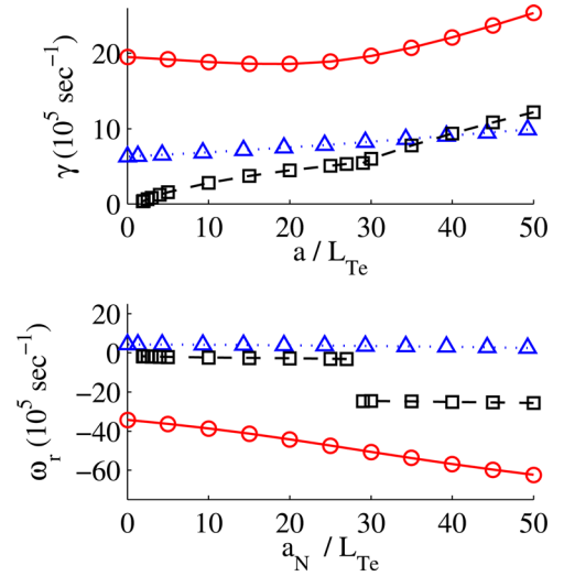
FIG. 14. (Color online) Variation from GS2 of \gamma and \omega_r with a_N/L_{Te} for the case of Fig. 2 with k_y\rho_i = 0.3983 . Circles: a_N/L_n = 52.4 , a_N/L_{Ti} = 0.0 ; triangles: a_N/L_n = 13.1 , a_N/L_{Ti} = 39.3 ; and squares: a_N/L_n = 0.0 , a_N/L_{Ti} = 0.0 .
