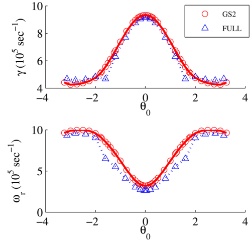
FIG. 6. (Color online) Variation of \gamma and \omega_r with \theta_0 at constant s=0.875 and \alpha = \pi/3 with \eta_i = \eta_e = 3 and k_y \rho_i = 0.3983 .
