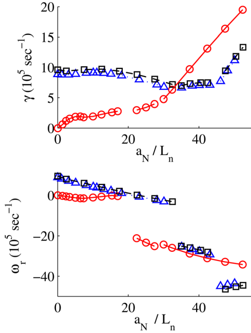
FIG. 12. (Color online) Variation of \gamma and \omega_r with a_N/L_n with k_y\rho_i = 0.3983 . Circles: a_N/L_T = 0.0 ; triangles: a_N/L_T = 39.3 ; and squares: a_N/L_T = 44.9 .
