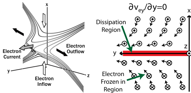
FIG. 10. Schematic from Yamada 12 showing electrons convecting the magnetic field lines out-of-plane (left) and a cut of this schematic in the inflow direction at z=0 near the X-point (right). For the figure on the right, circles represent magnetic field B_z and arrows represent electron flow for the portion of the inflow region ( x - y plane) near the X-point ( z=0 ) where electrons are frozen to the field lines. The horizontal red line at x=0 represents the electron dissipation region. Note that the figure on the left illustrates 2-D features of what could be a 3-D system; the figure on the right assumes a 2-D picture with no variation in the out-of-plane direction. Left panel reprinted with permission from M. Yamada, Phys. Plasmas 18 , 111212 (2011). Copyright 2011 American Institute of Physics.
