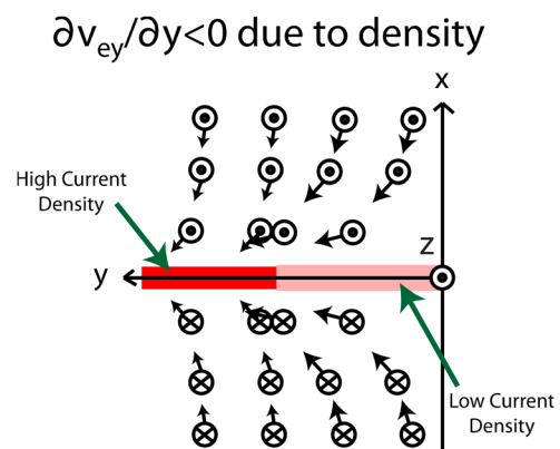
FIG. 12. Diagram showing how current density may build up in the y gradient region when \partial v_{ey}/\partial y < 0 due to density gradients. The buildup is due to a reduction in the reconnection rate in the gradient region by the mechanism described in the text.
