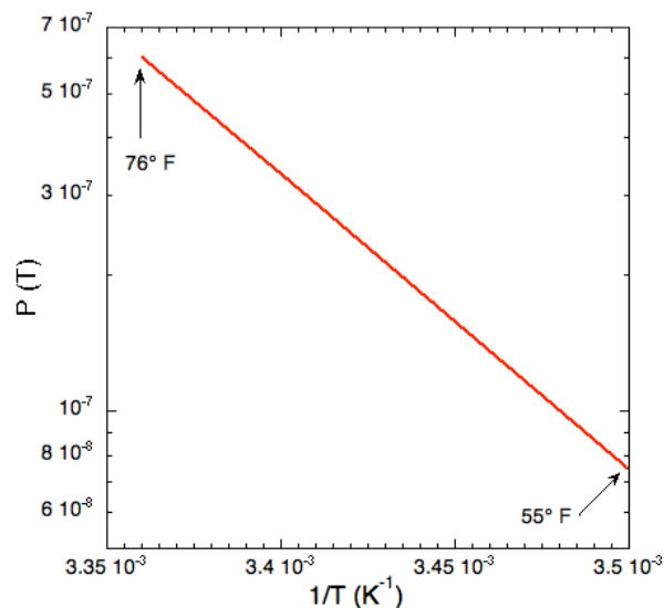
Figure 4. Dependence of vessel pressure on room temperature.
