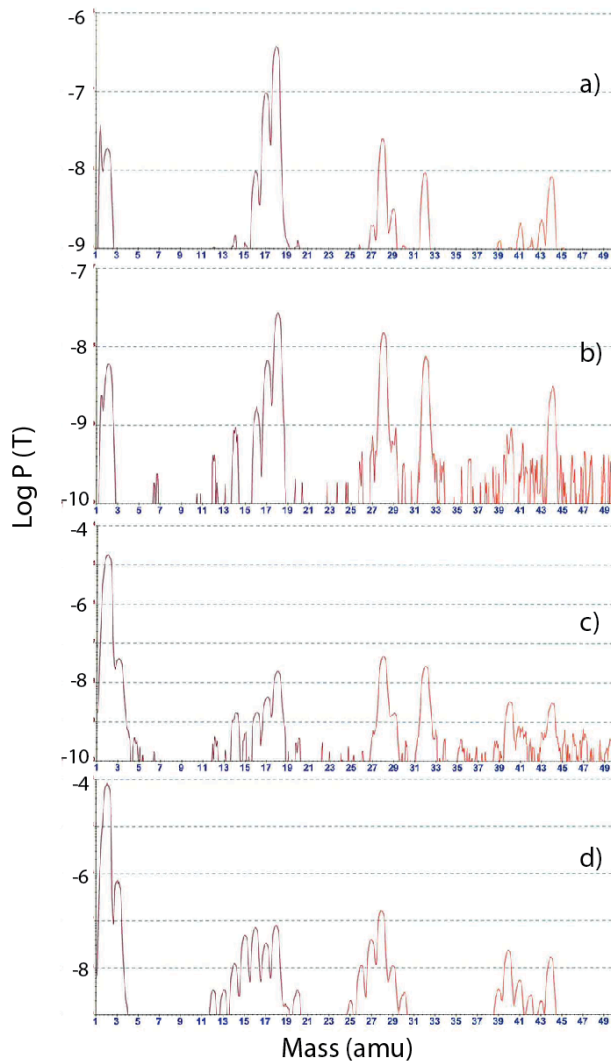
Figure 5. RGA spectra in the PFRC-2 for 4 cases on the same day, the first day the high-temperature superconducting flux conservers were cooled to LN2 temperature and the plasma pulse duration extended to 100 ms.
