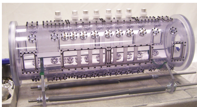
Figure 3. Assembled vacuum vessel. Note the polycarbonate end flanges, the black nylon screws, the black Viton seals for each port cover, and the eight polycarbonate quick disconnects epoxied to the top port covers.
