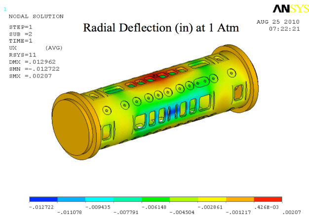
Figure 2. ANSYS prediction for the radial deflection of the PFC-2 polycarbonate vessel under 1 ATM pressure. Dimensions are in inches. The cylindrical pipe is 33" long, 10" OD with 5/8" wall.
