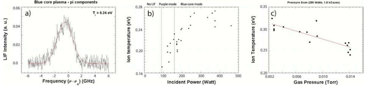
Fig. 2. (a) LIF intensity versus laser frequency, \nu , in the center of the MNX main chamber. \nu_0 is the frequency of the non-Doppler-shifted line. Uncertainty in the value of \nu_0 is 0.5 GHz. (b) T_{i,\perp} versus RF power. At this argon fill pressure, the plasma makes a transition from inductive (purple) to helicon (blue-core) mode at powers above 160 W. Though plasma exists at powers as low as 20 W, the LIF signal is too weak to provide a good measurement of ion temperature. (c) T_{i,\perp} versus argon fill pressure. (Color version available online at http://ieeexplore.ieee.org ).
