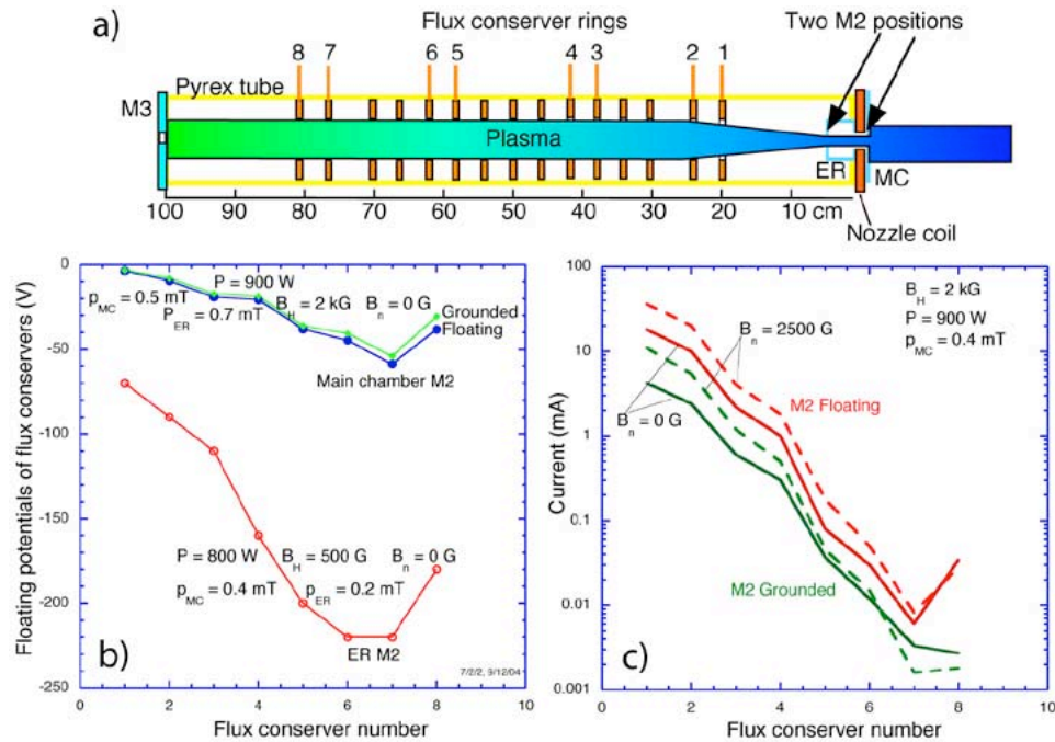
Fig. 9. (a) Schematic showing locations of 8 instrumented flux-conserver (copper) rings and the two positions of the M2 aperture plate used in this series of experiments. (b) Floating potentials of 8 instrumented flux-conserver rings for two different M2 positions. Nozzle field was zero. Adding a nozzle field approximately halves the amplitude of the floating potentials. (c) Current drawn by flux-conserver rings with and without the nozzle coil powered and with and without M2 grounded. MC M2 position was used.
