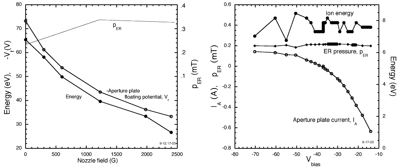
Fig. 8. (a) Dependence on nozzle-field strength of ER pressure, M2 floating potential and HEP E_z at z = 4 cm in the ER. (b) ER pressure, HEP E_z (at z = 3.2 cm) and M2 (aperture-plate) current versus bias voltage applied to M2. For geometry, see inset Fig. 5(b).
