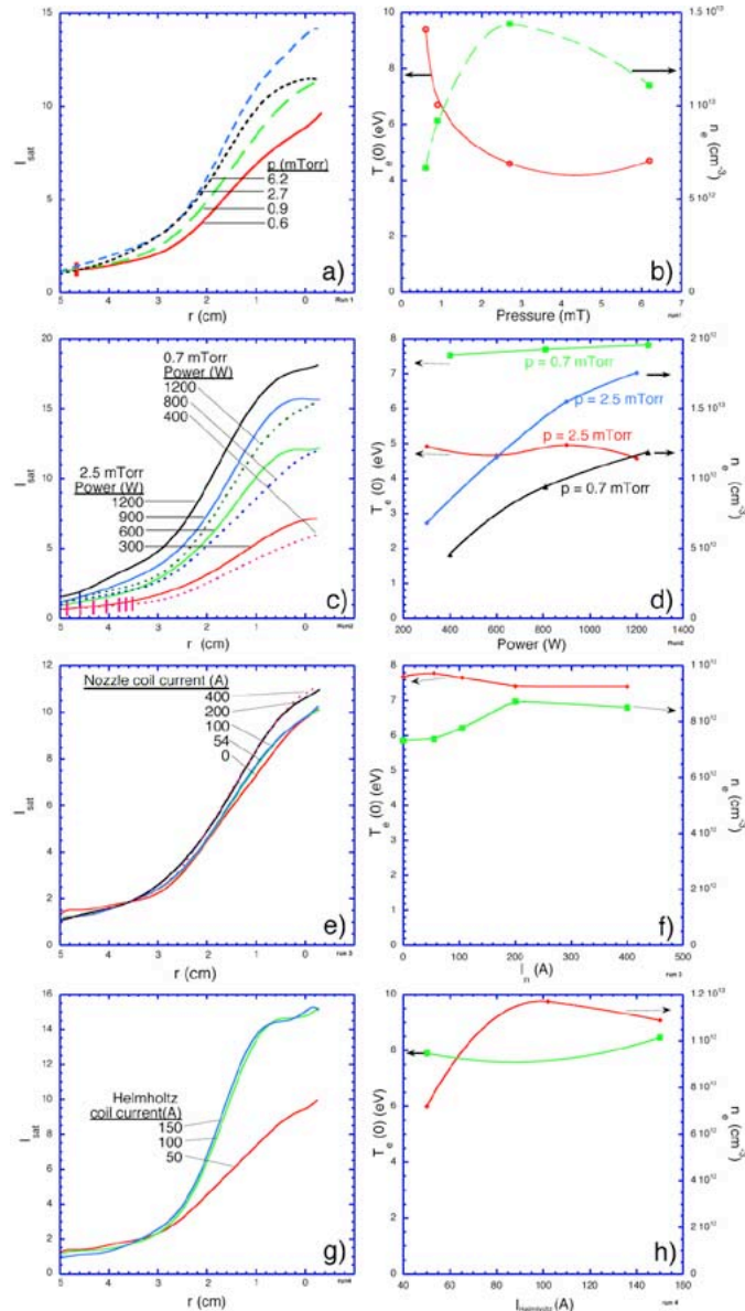
Fig. 6. Radial dependance of ion saturation current and dependences of central electron temperature and density of bulk plasma in center of MNX main chamber versus main chamber pressure, RF power, nozzle-coil current, and Helmholtz-coil current.
