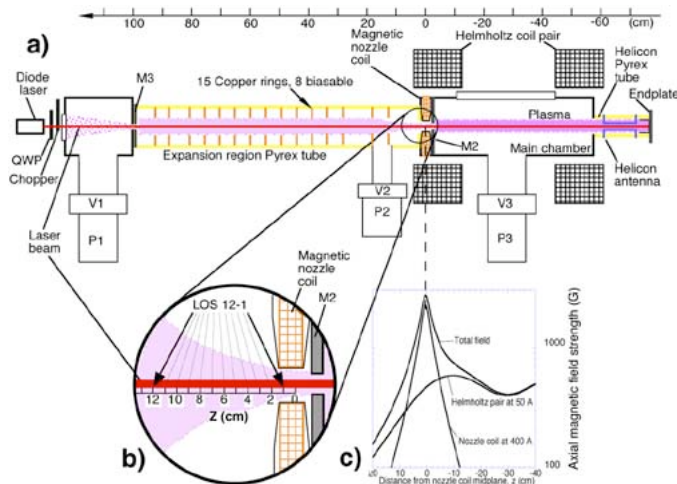
Fig. 1. Schematic of MNX. (a) Argon plasma is formed by absorption of helicon waves launched from a double-saddle antenna. Plasma flows through the main chamber along magnetic field lines created by a pair of Helmholtz coils. Plasma then flows through the aperture in M2 and the nozzle coil into the expansion region (ER). Beam of a diode laser is directed along the MNX axis. Scanning Langmuir probes are located in the center of main chamber and at z = 12, 24, and 70 cm in the ER. (b) LIF collection optics have 12 LOS intercepting axial points in the ER near the nozzle. Other LOS are in the main chamber. (c) On-axis axial magnetic field strength near the nozzle coil.
