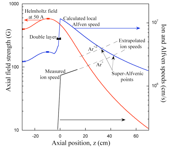
Fig. 12. Axial field strength (red), measured flow speed (black solid line), calculated Alfvén speed (blue) and extrapolated flow speeds (dashed black lines) for both Ar^+ and Ar^{+2} are shown. (Color version available online at http://ieeexplore.ieee.org ).
