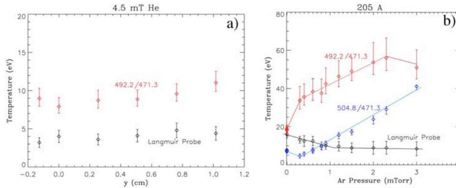
Fig. 11. (a) Radial profiles of T_e determined by the Sasaki et al. , [34] collisional-radiative model and with the Langmuir probe. (b) Dependence of three calculated electron temperatures, using probe data and the Sasaki method, on argon fill pressure in a helium helicon discharge. (Color version available online at http://ieeexplore.ieee.org ).
