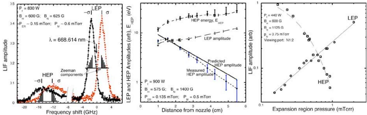
Fig. 4. (a) LIF amplitude versus frequency shift in the ER, 2 cm downstream from the nozzle midplane. Frequency zero is the non-Doppler-shifted line. Red (black) data are for RCP (LCP) laser beam. Six Zeeman + and -\sigma subcomponents merge into single peaks. Two sets of peaks are labeled, HEP and LEP. (b) HEP amplitude and E_z and LEP amplitude versus distance downstream from the nozzle coil. (c) HEP and LEP amplitudes versus argon pressure in the ER at 2 cm from the nozzle-coil midplane.
