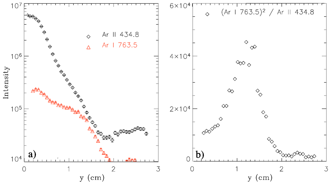
Fig. 10. (a) Abel-inverted brightnesses of an Ar I and an Ar II spectral line. (b) Ratio of brightnesses, (B_{ArI})^2 / B_{ArII} , as a function of radius. (Color version available online at http://ieeexplore.ieee.org ).
