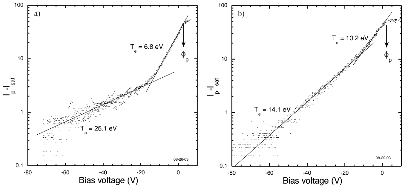
Fig. 7. Langmuir-probe characteristics in the ER. P_{RF} \sim 900 W, p_n \sim 0.7 mT, B_H \sim 700 G. (a) No nozzle field. (b) With 2-kG nozzle field. Error bars: \pm 3\% for bulk T_e ; \pm 20\% for tail T_e .
