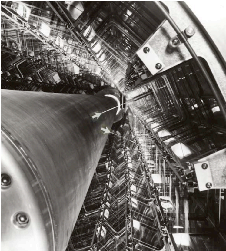
Figure 8: Inside of Astron tank—arrows point at resistive wires. (Lawrence Livermore National Laboratory Archives.)
