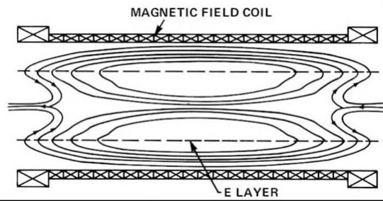
Figure 3: Formation of pattern of closed magnetic field lines in Astron. (Bromberg, 121.)
