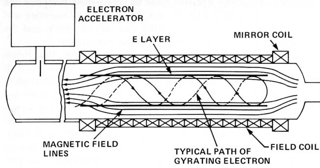
Figure 2: Gyration of E-layer electrons trapped in magnetic mirror field. (Bromberg, 121)
