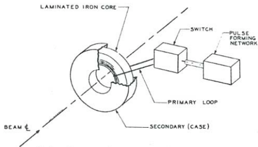
Figure 9: Induction acceleration principle. (Beal et al, "The Astron Linear Accelerator.")
