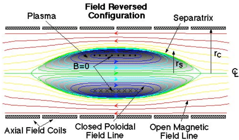
Figure 11: Formation of closed field lines in the FRC. ( http://www.aa.washington.edu/AERP/RPPL/programs/frc_intro.html )
