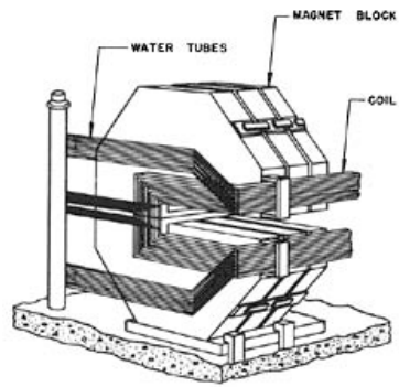
Figure 4: Schematic of Cosmotron magnet.( www.bnl.gov/bnlweb/history/cosmotron.asp )
