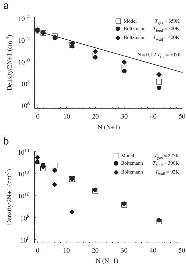
Fig. 7. Boltzmann plots of the ground state rotational distributions accounting for the combined effects of electron-impact excitation, wall collisions and feed gas rate for (a) the PFRC chamber and (b) the test cylinder within the PFRC chamber. Gas feed rate is 4 sccm, and 100 eV electrons at a density of 10^{12} \text{ cm}^{-3} .
