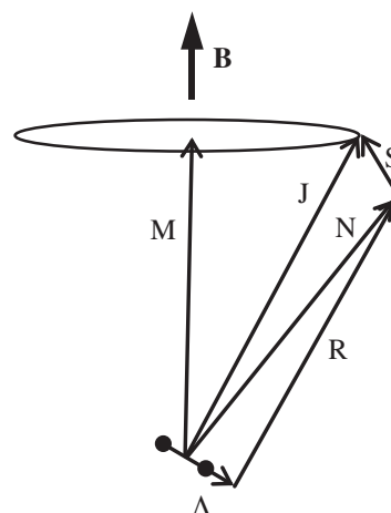
Fig. 2. Coupling of angular momentum vectors in the presence of magnetic field B for Hund's case (b) diatomic molecules.
