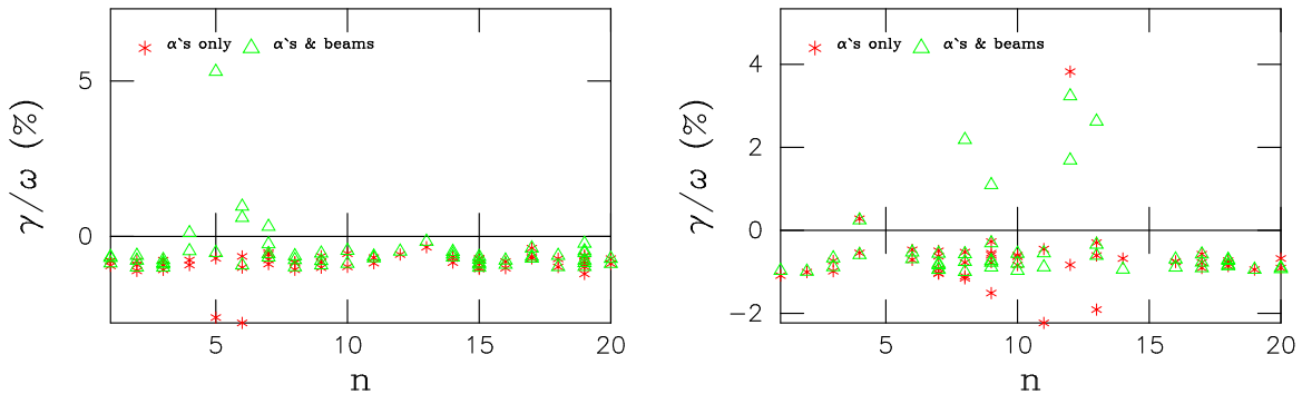
Figure 23: The same as in figure 22 but for Y = -20\text{cm} , #40500A06 run (left figure) and for the run #40500T02 with Y = -40\text{cm} (right figure).
