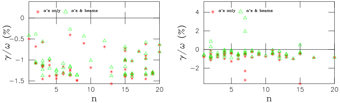
Figure 22: Toroidal mode number dependence of the AEs growth rates for the instabilities driven by alpha particles only (* points), and driven by both NBI ions and alpha particles ( \Delta points). Results are for NBI aiming Y = 20\text{cm} above plasma axis, ITER TRANSP run #40500T04 (left figure) and for the run #40500T03 with Y = 10\text{cm} (right figure).
