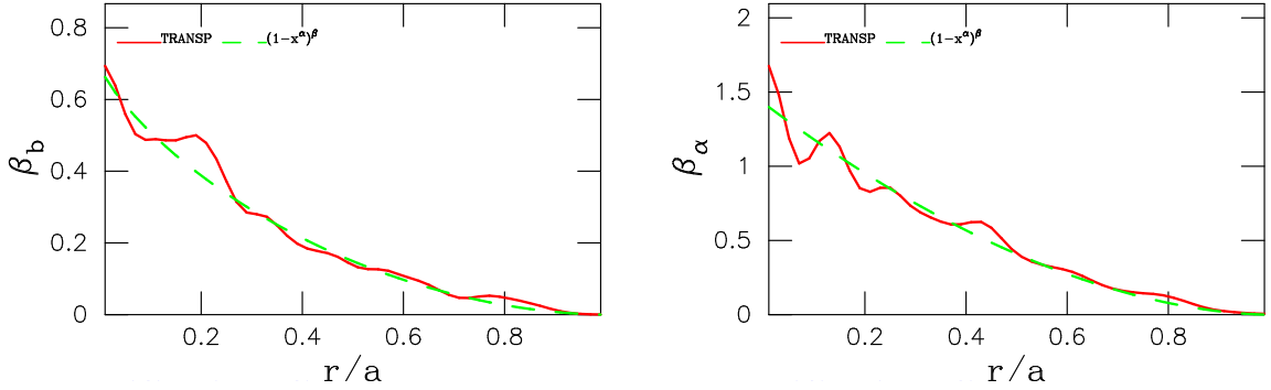
Figure 21: Example of the TRANSP produced NBI (left) and fusion alphas (right) beta profiles (in %) for ITER hybrid plasma run 40500T04. Shown as solid lines are the profiles from TRANSP code. Shown as dashed lines are the fitted profiles, used in NOVA simulations.
