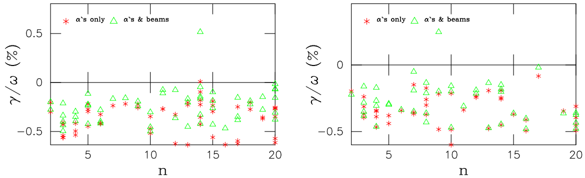
Figure 17: The same as in figure 16 but for Y = -20 , #20100T03 run (left figure) and for the run #20100T02 with Y = -38\text{cm} (right figure).
