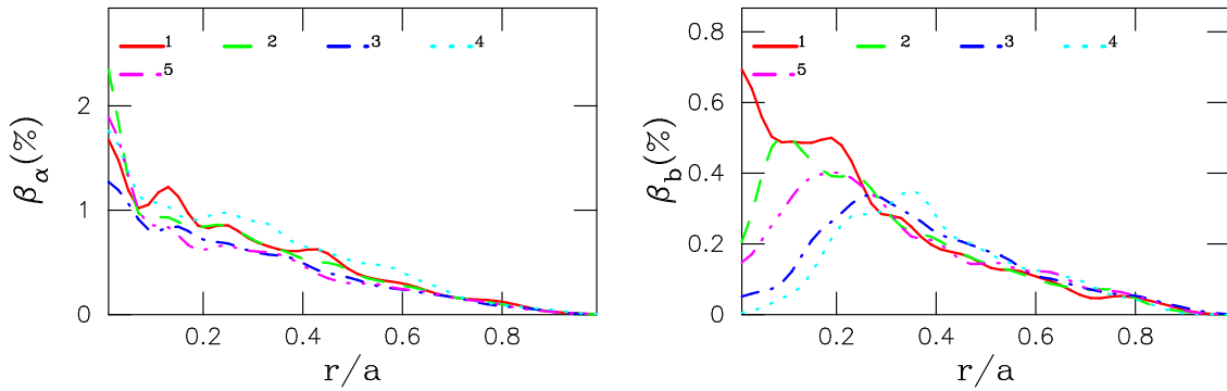
Figure 8: Fusion alphas and NNBI confined ion betas for Hybrid scenario ITER plasmas.
