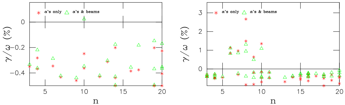
Figure 16: Toroidal mode number dependence of the AEs growth rates for the instabilities driven by alpha particles only (* points), and driven by both NBI ions and alpha particles ( \Delta points). Results are for on-axis Y = 0 NBI, ITER TRANSP run #20000T01 (left figure) and for the run #20000T02 with Y = -10 cm (right figure).
