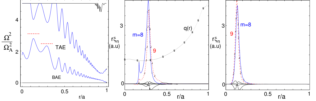
Figure 20: Ideal MHD n = 7 continuum for ITER hybrid plasma run #40500t03 (left figure) and two most unstable low shear localized TAE poloidal harmonic radial structures for the case with NBI aiming 10cm above the magnetic axis. Center figure represents the radial structure of TAE with \Omega^2/\Omega_A^2 = 2.41 and right figure corresponds to TAE with \Omega^2/\Omega_A^2 = 3.09 , where NOVA uses normalization \Omega_A = v_{A0}/q_a R . The radial extent of these modes is shown in the left figure as dashed lines. Vertical position of these lines corresponds to the normalized eigenfrequency.
