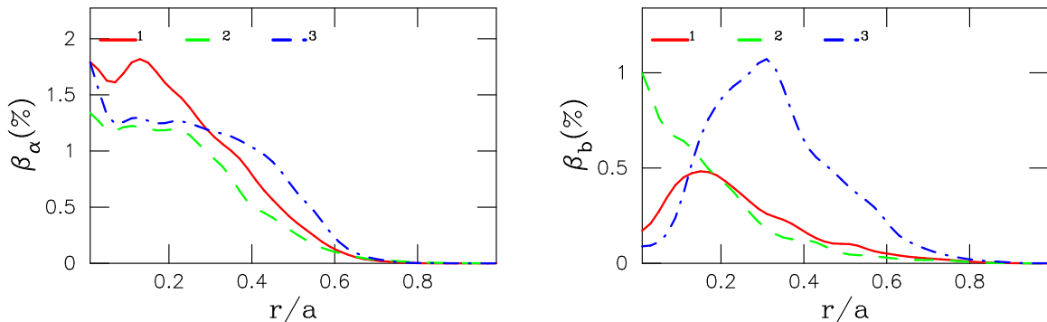
Figure 12: Fusion alphas, \beta_\alpha , and NNBI confined ion, \beta_b , betas.
