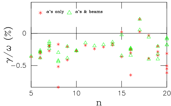
Figure 24: The same as in figure 22 but for Y = 3cm (on-axis heating), #40500.A04 run.
