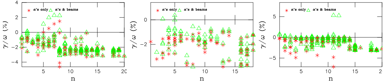
Figure 27: Toroidal mode number dependence of the AEs growth rates for the instabilities driven by alpha particles only (* points), and driven by both NBI ions and alpha particles ( \Delta points). Results are for ITER reversed shear plasmas numbered #1, 2, 3 listed in table IV, shown in left, center and right figures, respectively.
