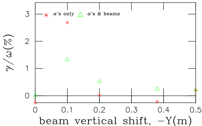
Figure 19: Most unstable TAE growth rates vs. vertical deviation of the beam injection from the magnetic axis.
