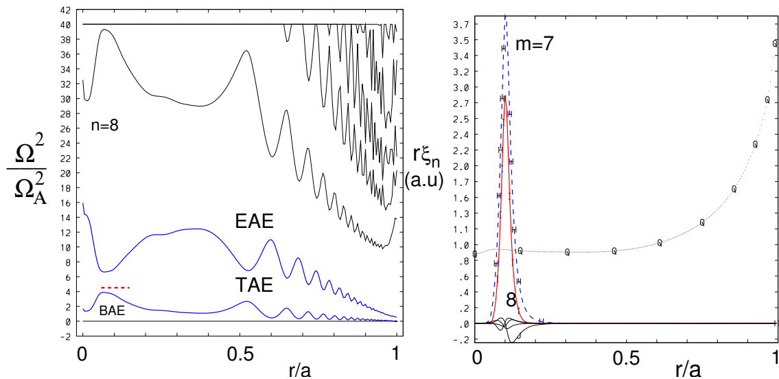
Figure 14: Ideal MHD continuum for ITER normal shear H-mode plasma run #20000T02 (left figure) and the most unstable core localized TAE poloidal harmonic radial structure for this case with NBI aiming 10cm below the magnetic axis. The radial extent of this mode is shown in the left figure as a dashed line corresponding to the normalized TAE eigenfrequency.
