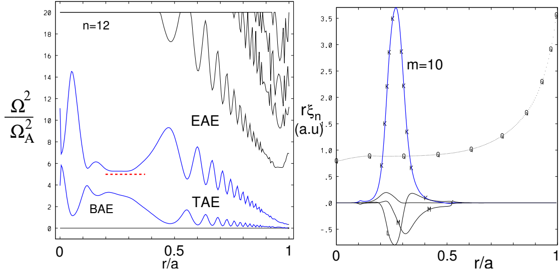
Figure 15: Ideal MHD continuum for ITER normal shear H-mode plasma run #20100T03 (left figure) and the unstable low shear localized TAE poloidal harmonic radial structure for this case with NBI aiming 20cm below the magnetic axis. The radial extent of this mode is shown in the left figure as a dashed line corresponding to the normalized TAE eigenfrequency.
