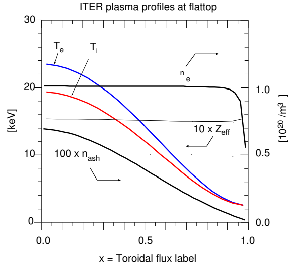
Figure 4: Profiles of the ITER H-mode plasma. The \text{He}^4 ash density times 100 is computed from the fast alpha thermalization assuming R_{ash} = 20\% and D_{ash} = 0.8 [\text{m}^2/\text{s}] , and is in steady state at the time shown.
