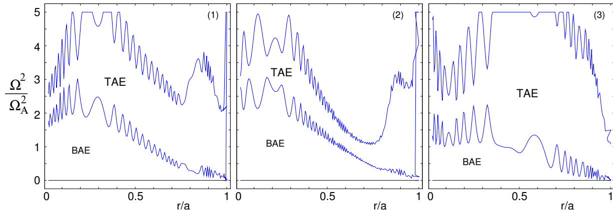
Figure 26: Ideal MHD n = 10 continuum for ITER reversed shear plasmas numbered #1, 2, 3 in table IV. Frequencies are normalized to \Omega_A = v_{A0}/q_a R .
