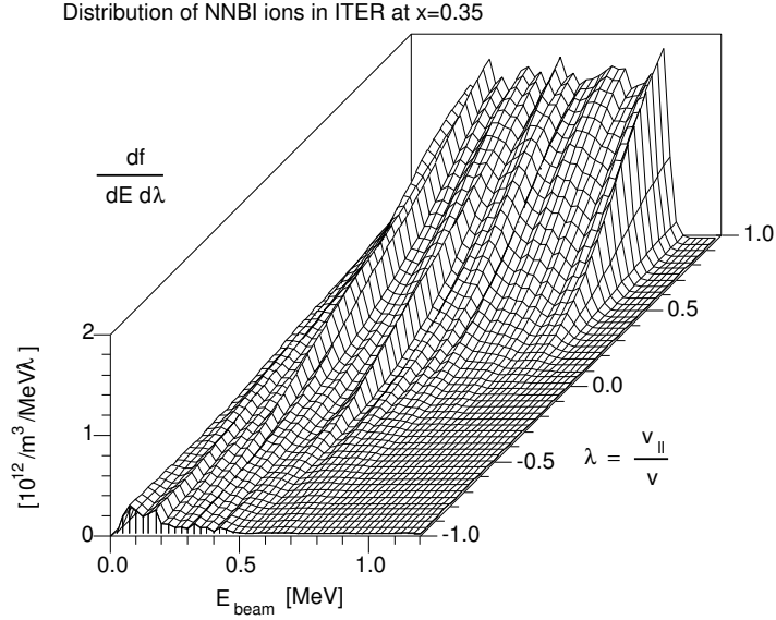
Figure 6: Distribution of the ITER NNBI beam ions in energy and pitch angle at x = 0.35 , averaged over poloidal angle, computed by the TRANSP Monte Carlo model. The neutrals are injected at 1MeV with v_{||}/v \simeq 1 , and the beam ions become more isotropic as they slow down.
