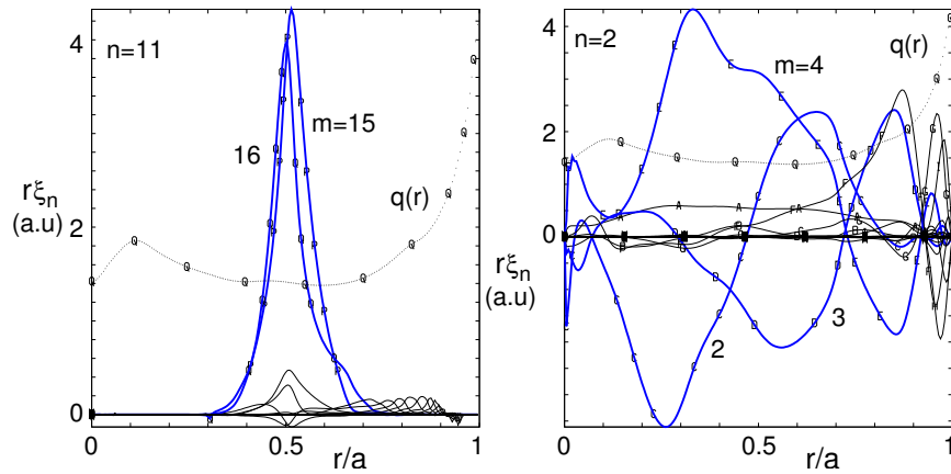
Figure 28: Left figure represents the radial structure of the most unstable localized TAE in strongly reversed ITER AT plasma #3. Left figure TAE has n = 11 and \Omega^2/\Omega_A^2 = 2.12 . Right figure corresponds to EAE with \Omega^2/\Omega_A^2 = 6.7 and n = 2 , which is weakly unstable, but more global.
