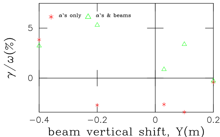
Figure 25: Most unstable TAE growth rates vs. vertical deviation of the beam injection from the magnetic axis for hybrid plasma.
