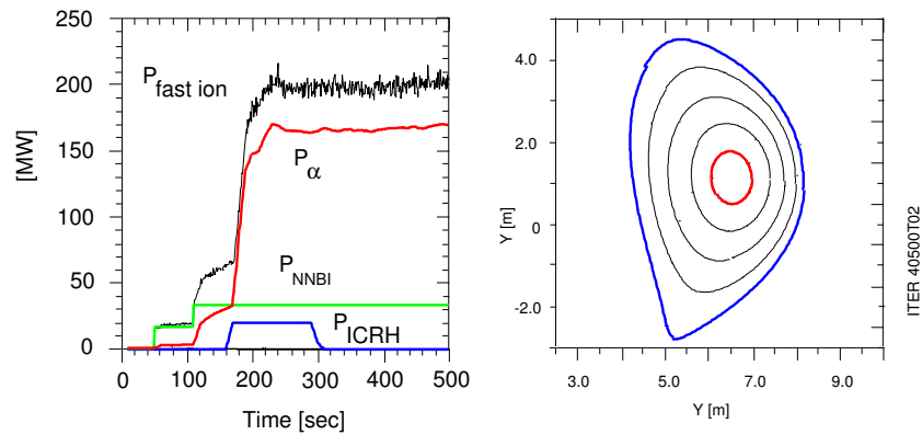
Figure 9: a) Heating powers from fusion alpha particles, NNBI, and ICRH, b) Poloidal section showing surfaces of constant toroidal flux.
