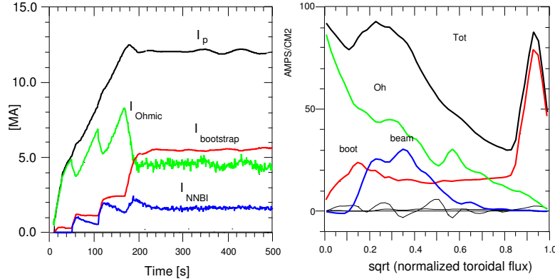
Figure 10: a) Plasma currents and b) profiles in an ITER Hybrid plasma.
