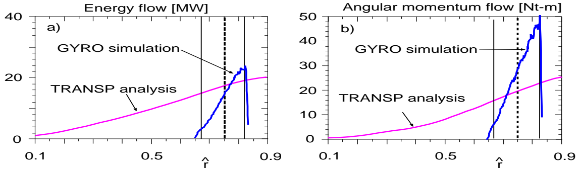
Figure 2: Profiles of a) total energy and b) angular momentum flow for JET 42982 from the TRANSP analysis and GYRO simulation
