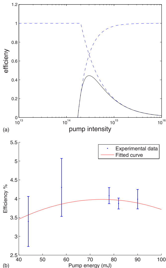
FIG. 7. (Color online) The upper plot shows a theoretically estimated efficiency of BRA as described above. It has well defined maximum at a certain pump intensity. The lower plot shows experimentally measured dependence of the BRA efficiency vs the pump energy (Ref. 14). The intensity of the pump is proportional to the pump energy since the other parameters of the pump are fixed. The solid line is the least square parabolic fit of the experimental data points.
