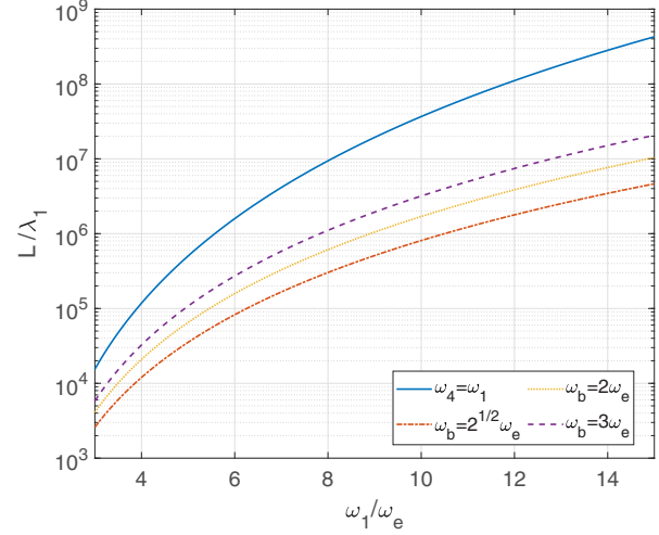
FIG. 4. The exponentiation length L to the laser wavelength \lambda_1 , as a function of the laser-to-plasma frequency ratio \omega_1 / \omega_e , for the regimes (5) and (8)–(9) at |a_4|^2 = |a_1|^2 = 0.1 .
