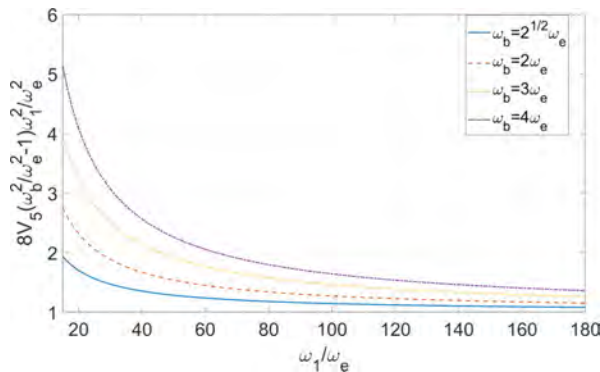
FIG. 5. Far asymptotic behavior of the six-photon coupling coefficient V_5 in the regimes (8)–(9).
