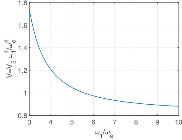
FIG. 3. The six-photon coupling coefficient V = V_5 \omega_1^4 / \omega_e^4 as a function of the laser-to-plasma frequency ratio \omega_1 / \omega_e for the regime (5).
