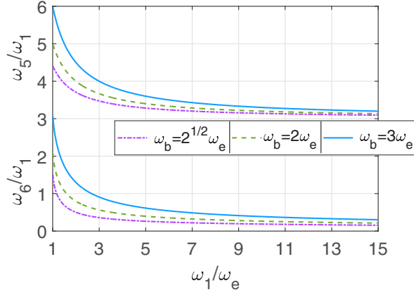
FIG. 2. Frequency multiplication factors \omega_5/\omega_1 and \omega_6/\omega_1 as functions of \omega_1/\omega_e in six-photon scattering of three photons of frequency \omega_1 and a photon of frequency \omega_4 into a photon of frequency \omega_5 and a photon of frequency \omega_6 = \omega_4 - \omega_b , for a few values of parameter \omega_b/\omega_e = \sqrt{2} , 2, and 3.
