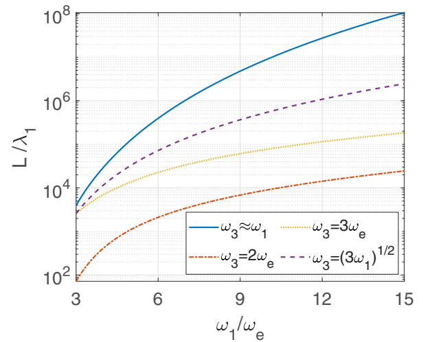
FIG. 6. The exponentiation length L ratio to the laser wavelength \lambda_1 , as a function of the laser-to-plasma frequency ratio \omega_1/\omega_e , for the regimes (10) at |a_3|^2 = |a_1|^2 = 0.1 and a few different \omega_3 . The solid line corresponds to \omega_3 close to, but different from \omega_1 . This line is nearly the same as one obtained by formally replacing in the regime (5) |a_1|^4 for 6|a_1|^2|a_3|^2 , so that at |a_3|^2 = |a_1|^2 the resulting L is six times smaller than in the regime (5).
