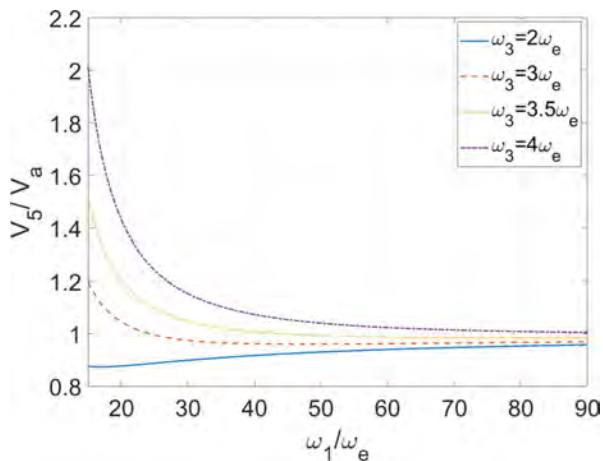
FIG. 7. Far asymptotic behavior of the six-photon coupling coefficient V_5 in the regimes (10).
