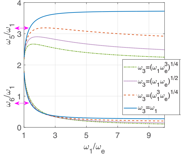
FIG. 1. Frequency multiplication factors \omega_5/\omega_1 and \omega_6/\omega_1 as functions of \omega_1/\omega_e in six-photon scattering of two photons of frequency \omega_1 and two photons of frequency \omega_3 into a photon of frequency \omega_5 > 2\omega_1 and a photon of frequency \omega_6 < 2\omega_1 .
