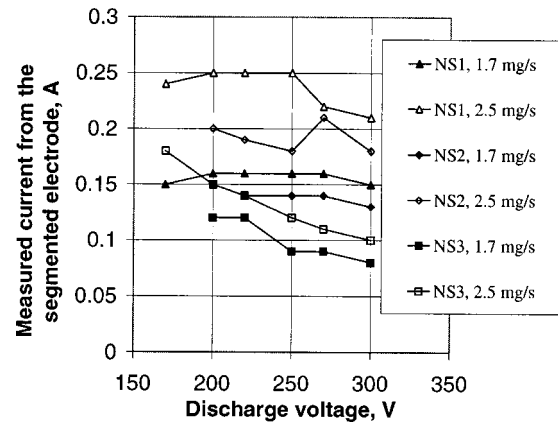
FIG. 12. Current to the segmented electrode, measured for three segmented electrode configurations, NS1, NS2, and NS3 (under cathode bias) measured at two mass flow rates 1.7 and 2.5 mg/s.
