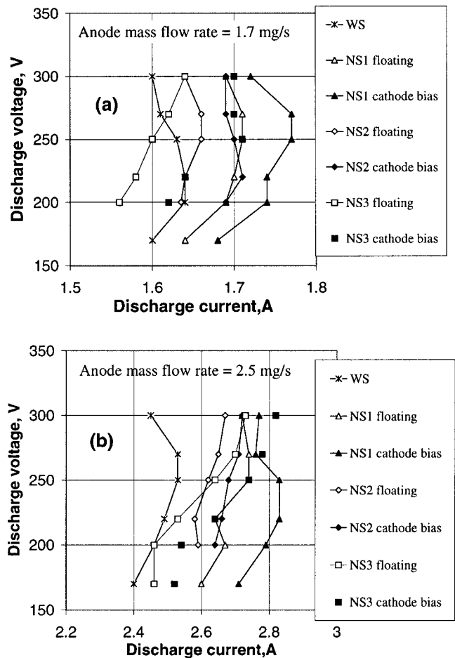
FIG. 7. V-I characteristics of the thruster for the seven thruster configurations: WS; and NS1, NS2, and NS3 (floating and under cathode bias) at 1.7 mg/s (a) and 2.5 mg/s (b).
