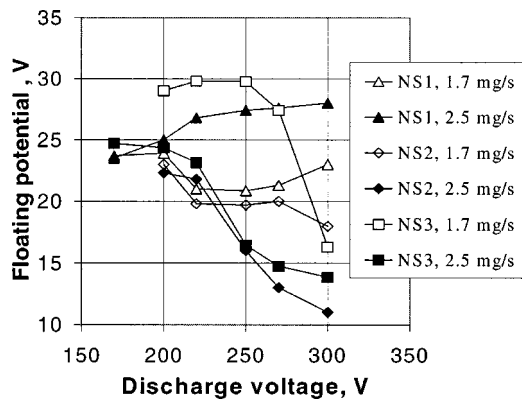
FIG. 13. Floating potential measured between the cathode and segmented electrode for three segmented electrode configurations NS1, NS2, and NS3 at two mass flow rates 1.7 and 2.5 mg/s.
