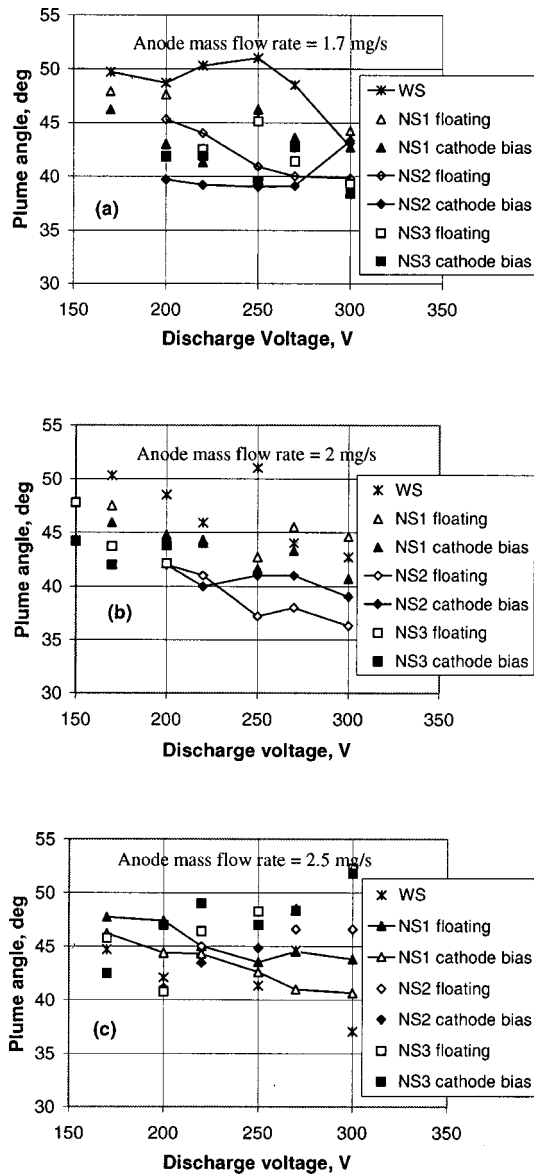
FIG. 11. Half-plume angle estimated for 90% of the measured ion flux from the thruster of different configurations (WS, NS1, NS2, and NS3, floating, biased) at three different mass flow rates.
