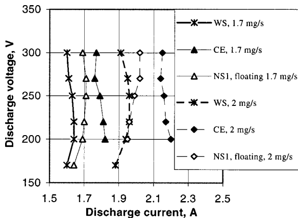
FIG. 9. V-I characteristics for three thruster configurations WS, NS1 (floating and under cathode bias), and CE, at 1.7 and 2 mg/s.
