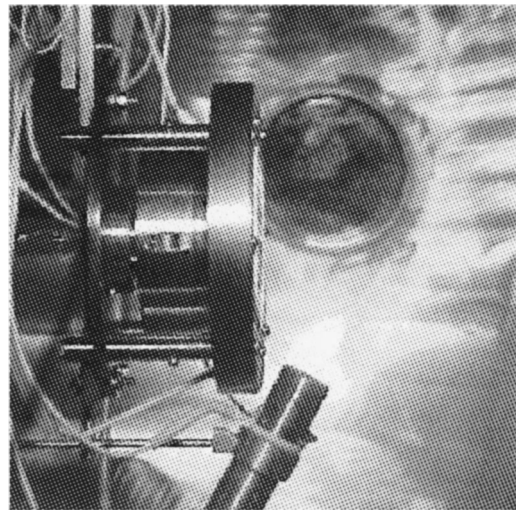
FIG. 2. PPPL model Hall thruster.
