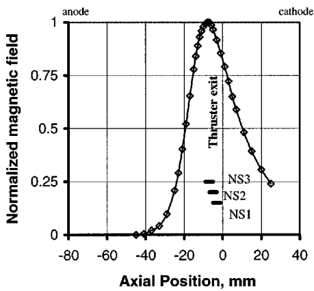
FIG. 4. Normalized measured profile of the radial component of the magnetic field along the thruster axis near the channel median at electromagnet coils current of 2 A. NS1, NS2, NS3, are locations of inner-segmented electrodes along the thruster axis.
