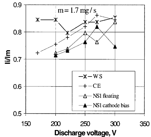
FIG. 10. Propellant utilization vs discharge voltage measured for four thruster configurations WS, NS1 (floating and under cathode bias), and CE at 1.7 mg/s.
