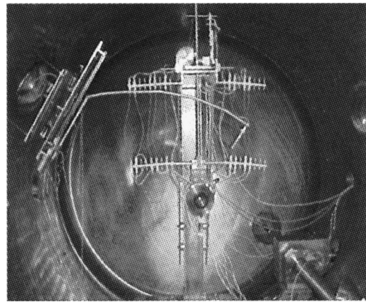
FIG. 6. Thrust stand and probe setup.
