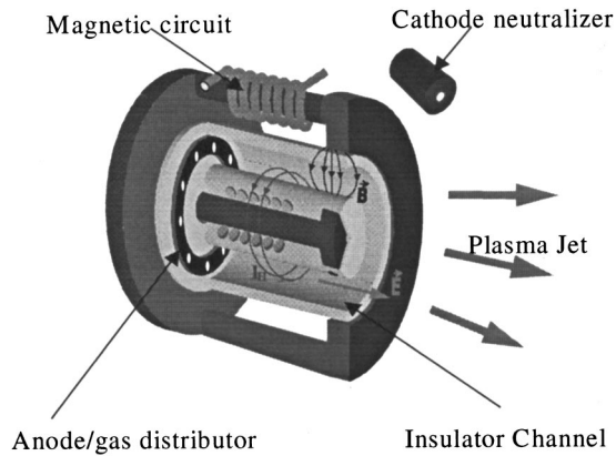
FIG. 1. Schematic drawing of the Hall thruster.
