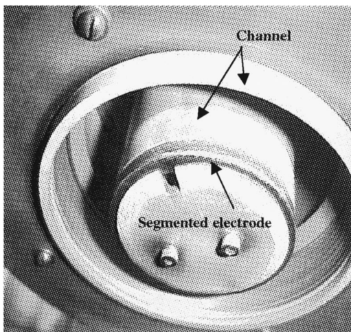
FIG. 5. Negative side (NS) segmented electrode attached to the inner wall of the ceramic channel.
