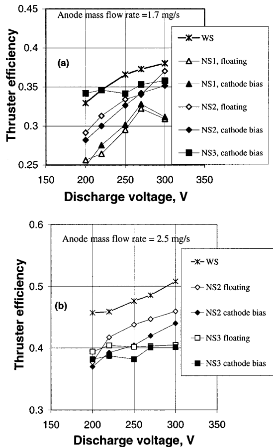
FIG. 15. Thruster efficiency vs discharge voltage measured for WS and NS1, NS2, and NS3 floating and biased configurations at two mass flow rates: 1.7 mg/s (a) and 2.5 mg/s (b).
