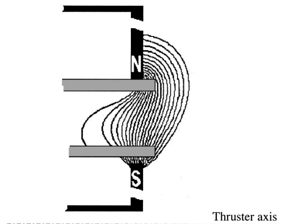
FIG. 3. Simulated magnetic field.
