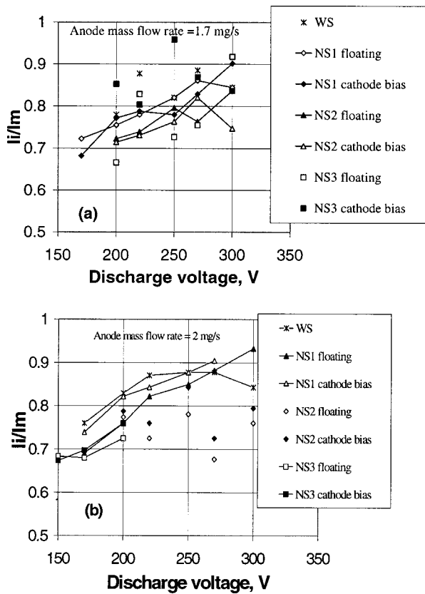
FIG. 8. Propellant utilization vs the discharge voltage measured for the seven thruster configurations WS, NS1, NS2, and NS3 (floating and under cathode bias) at 1.7 mg/s (a) and 2 mg/s (b).
