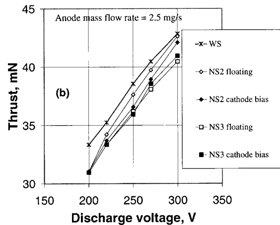
FIG. 14. Thrust vs discharge voltage measured at two mass flow rates, 1.7 mg/s for WS, NS1, NS2, and NS3 (a) and 2.5 mg/s for WS, NS2, and NS3 (b).
