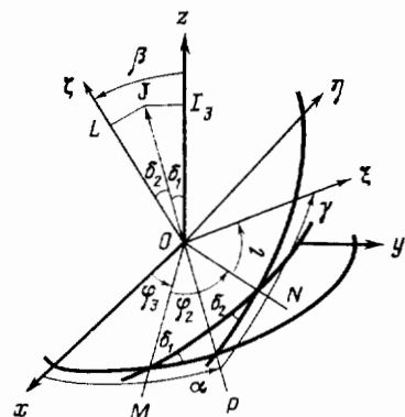
FIG. 2. Mutual placement of the laboratory (x, y, z) and the molecular (\xi, \eta, \zeta) coordinate systems: \alpha, \beta, \gamma are the Euler angles, and l, \varphi_2, \varphi_3 are the Deprit angle variables ( OP is the line of nodes, OM \perp J , ON \perp J ).
