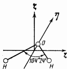
FIG. 1. Choice of the molecular coordinate system for the water molecule.
