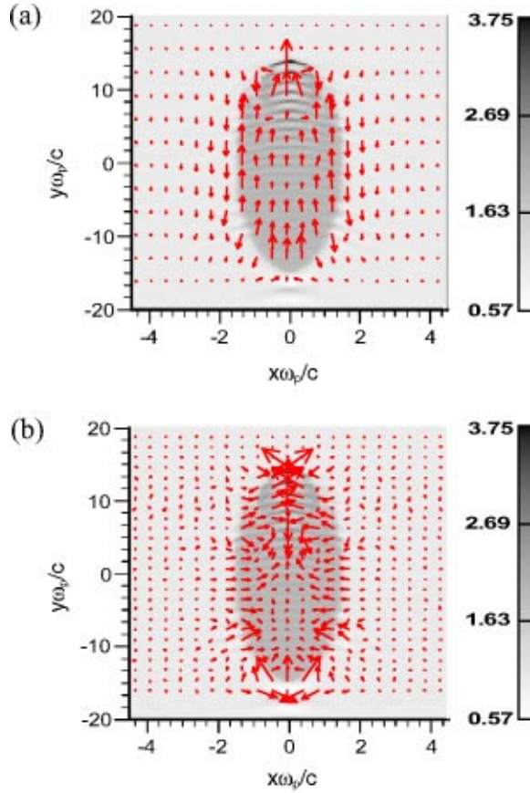
FIG. 2. (Color online). The excitation of plasma waves by the beam head is calculated in two-dimensional slab geometry using the EDPIC code (Ref. 14) for the following beam parameters: V_b = 0.5c , Z_b = 1 , n_b = n_p , l_b/r_b = 10 , and l_b = 15c/\omega_p . Shown in the figure are electron charge density contour plots in (x\omega_p/c, y\omega_p/c) space and the vector fields for (a) the total current, and (b) minus the electric field, -E .
