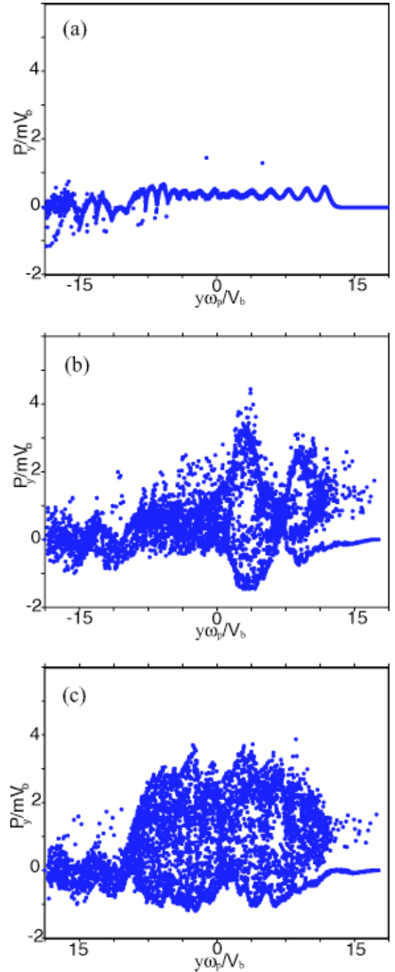
FIG. 3. (Color online). Electron phase space for 1D PIC simulations of the beam entering the plasma at t = 0 . Here, V_b = 0.5c , Z_b = 1 , l_b = 7.5c/\omega_p , and (a) n_b = n_p ; (b) n_b = 2n_p ; and (c) n_b = 2n_p . The steady state establishes after the beam enters the plasma in case (a). Under these circumstances, the plasma phase space also shows applicability of the fluid approximation. However, in case (b) the plasma wave breaks and the electrons are heated by wave-particle interactions. In this situation, the cold-fluid approximation is not applicable. Moreover, the phase space slowly evolves with time as shown. The times after entering the plasma correspond to (b) t = 113/\omega_p , and (c) t = 245/\omega_p .
