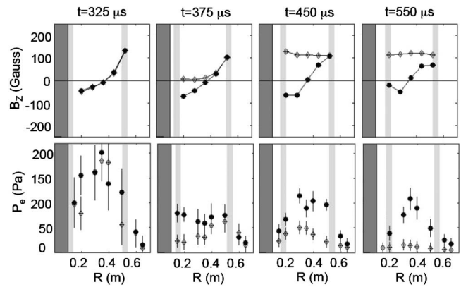
FIG. 4. Radial profiles of the axial magnetic field (top row), as measured by the spoke probes, and electron pressure (bottom row), as measured by radially scanning a Langmuir probe at the midplane. Results are shown for argon discharges with (closed symbols) and without (open symbols) inductive sustainment.
