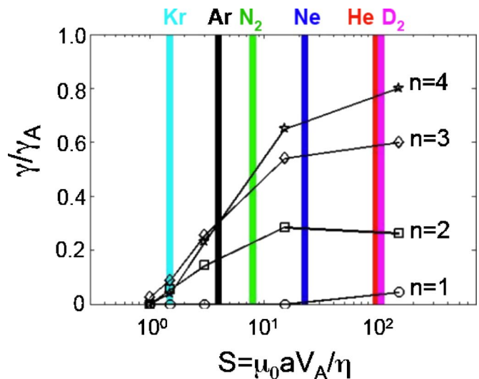
FIG. 12. (Color online) Growth rates for the n=1, 2, 3 , and 4 axially polarized co-interchange modes, as a function of Lundquist number. The vertical lines show the typical Lundquist numbers of the different working gases.
