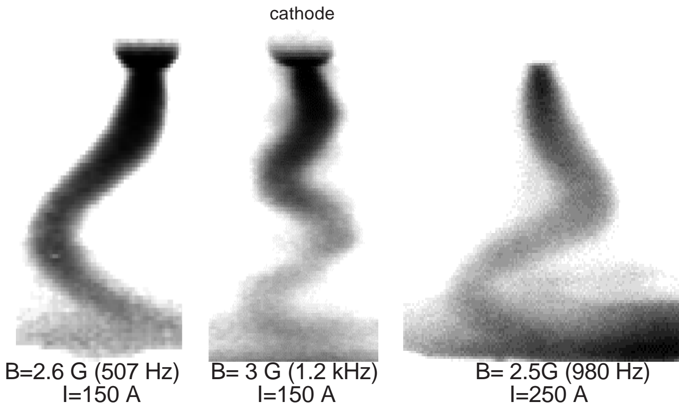
Fig. 4: Sample images of the externally driven oscillatory motion of the arc at different frequencies and applied AC magnetic fields. The geometry and camera set-up is the same as figure 3. The axial wavelength is shorter for higher applied frequencies, as shown by the comparison between the left and middle images, and the wavelength increases with increasing current, as shown by the comparison between the middle and right images. At each vertical position the arc oscillates horizontally in time at the applied frequency.
