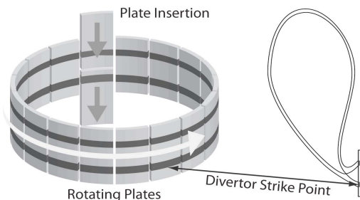
Figure 1 - Conceptual design of a moving divertor plate system in a tokamak. The plates form a ring around the bottom of the tokamak, with the divertor strike zones indicated by the dark bands. The plates could be inserted and removed vertically, and could also be moved toroidally.
