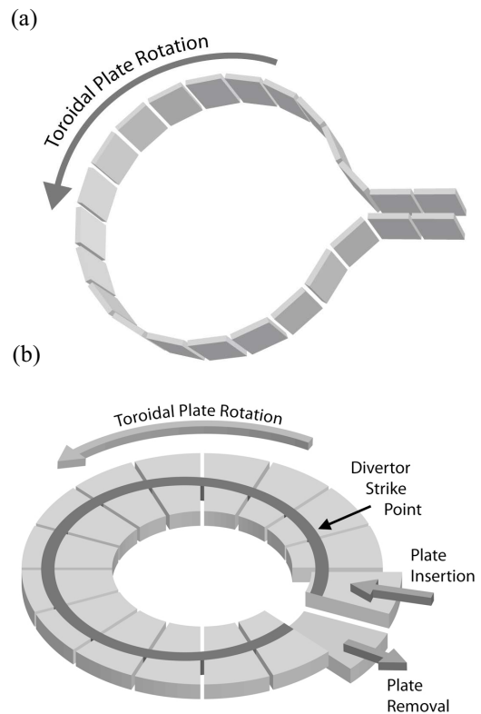
Figure 3 - Alternative methods for plate location and motion in which some of the plasma strike zone is allowed to become uncovered. In (a) the plates are vertical and enter and exit the tokamak in a continuous toroidal loop. In (b) the horizontal plates are replaced with a radial motion and rotated in an offset toroidal direction to sweep the heat flux over the plate radius.
