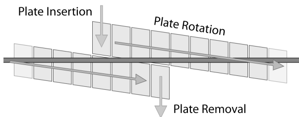
Figure 2 – Method to sweep the plates both in both the toroidal and vertical directions simultaneously in order to reduce the number of plate exchange locations inside the tokamak. The toroidal direction is horizontal in this 2-D view, and a plasma strike zone is shown as a dark line. The arrows show the directions of plate insertion, toroidal rotation, and removal.
