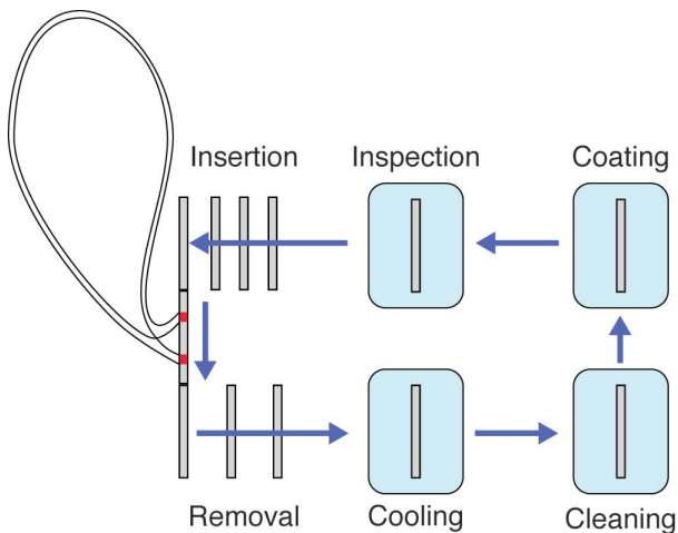
Figure 4 – Plate processing outside the tokamak. Once the plates are removed from the main chamber they can be processed and returned in optimum condition. External processing would also allow rapid testing of redesigned divertor plates.
