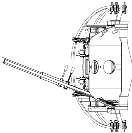
Figure 5 - Conceptual sketch of a movable divertor module for NSTX-U. A single divertor segment can be removed between shots, and moved radially during a shot using a long bellows.
