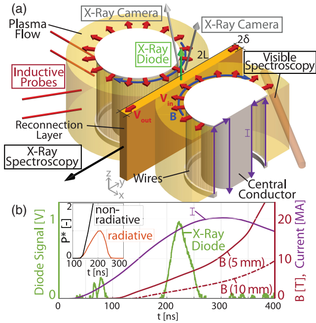
FIG. 1. (a) A three-dimensional model of the dual wire array load and diagnostic setup. (b) Current (purple), x-ray diode signal (green), and magnetic field at 5 and 10 mm from the wires (red). Inset: Simulated x-ray emission from the reconnection layer, filtered with 8 \mu\text{m} Be, for non radiative (black) and radiatively cooled (orange) cases. X-ray power P^* is normalized using the peak power in the radiatively cooled simulation.
