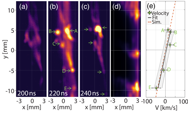
FIG. 2. (a)–(c) Time-gated x-ray images (10 ns exposure) of the reconnection layer, showing hot spots (green arrows) inside a bright elongated layer. (d) Synthetic x-ray image of the layer obtained by postprocessing a 3D simulation at 220 ns with x-ray emission and radiation transport modeling [36]. (e) Velocity of the hot spots inside the reconnection layer. The solid line is a linear fit to the hot spot velocity, and dashed orange line is the simulated outflow velocity in the reconnection layer, averaged between 200 and 250 ns.
