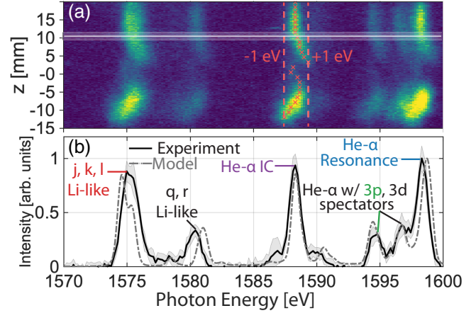
FIG. 3. (a) Time-integrated x-ray spectra from the reconnection layer showing Al K-shell emission. Red crosses show the position of the He- \alpha intercombination line. (b) X-ray spectrum averaged over z = (10 \pm 1) mm [white line in (a)] showing He-like and Li-like satellite transitions (black), and calculated spectrum from the SCRAM and radiation transport model for 170 eV, 1 \times 10^{18}\ \text{cm}^{-3} hot spot density, and 0.5 mm hot spot size (gray dashed).
