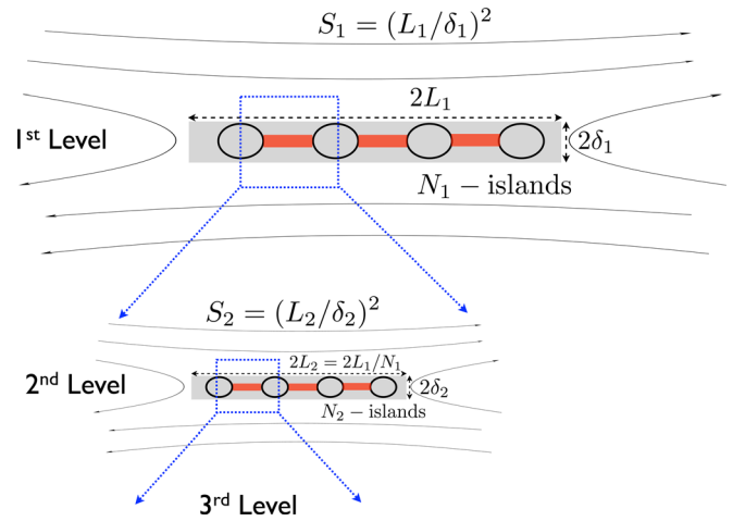
FIG. 2. (Color online) In the regimes of high Lundquist number and large plasma size, the plasmoid instability gives rise to a hierarchy of interacting current sheets and islands. The above sketch gives the notation used here for describing this hierarchy.
