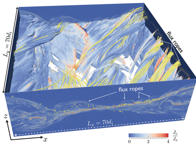
FIG. 4. (Color) Results from a kinetic simulation (Ref. 65) of guide field reconnection showing the formation and interaction of flux ropes as illustrated by an isosurface of the particle density colored by the magnitude of the current density along with sample magnetic field lines (yellow). Simulation parameters are m_i/m_e = 100 with the initial guide field equal to the reconnecting field. The domain size is 70d_i \times 70d_i \times 35d_i corresponding to 2048 \times 2048 \times 1024 cells and \sim 10^{12} particles.
