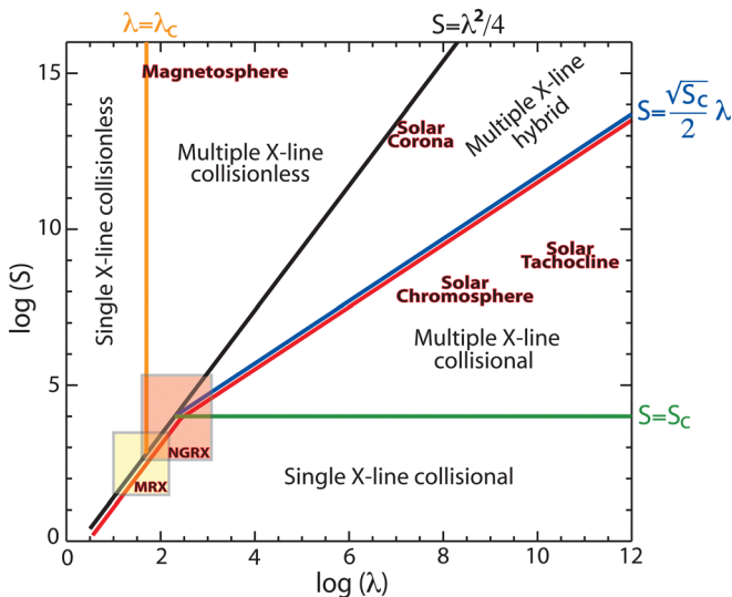
FIG. 1. (Color online) A phase diagram for magnetic reconnection in two dimensions. If either S or the normalized size, \lambda , is small, reconnection with a single X-line occurs in collisional or in collisionless phases. When both S and \lambda are sufficiently large, three new multiple X-line phases appear with magnetic islands. The dynamics of new current sheets between these islands are determined either by collisional physics or by collisionless physics (see Secs. III and IV). The conditions for electron runaway are shown as red lines (see Sec. V). The locations for reconnection in Earth’s magnetosphere, solar corona, solar chromosphere, and solar tachocline are also shown. The existing experiments, such as MRX, do not have access to these new phases. A NGRX is required for such accesses to these new phases directly relevant to reconnection in heliophysical and astrophysical plasmas.
