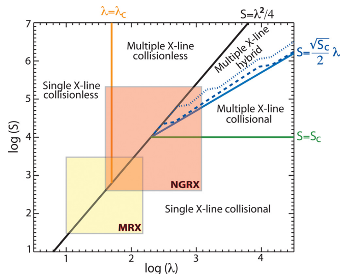
FIG. 3. (Color online) The phase diagram in a smaller parameter space to show dotted and dashed lines better (see texts in Sec. III). Other symbols are same as in Fig. 1.
