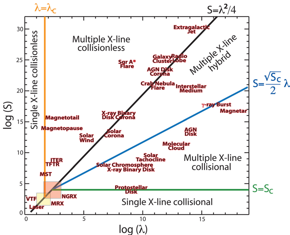
FIG. 5. (Color online) Various laboratory, heliophysical, and astrophysical plasmas, in which magnetic reconnection is believed to occur, are shown in the phase diagram. Other symbols are same as in Fig. 1. See the text and Table 1 for details.
