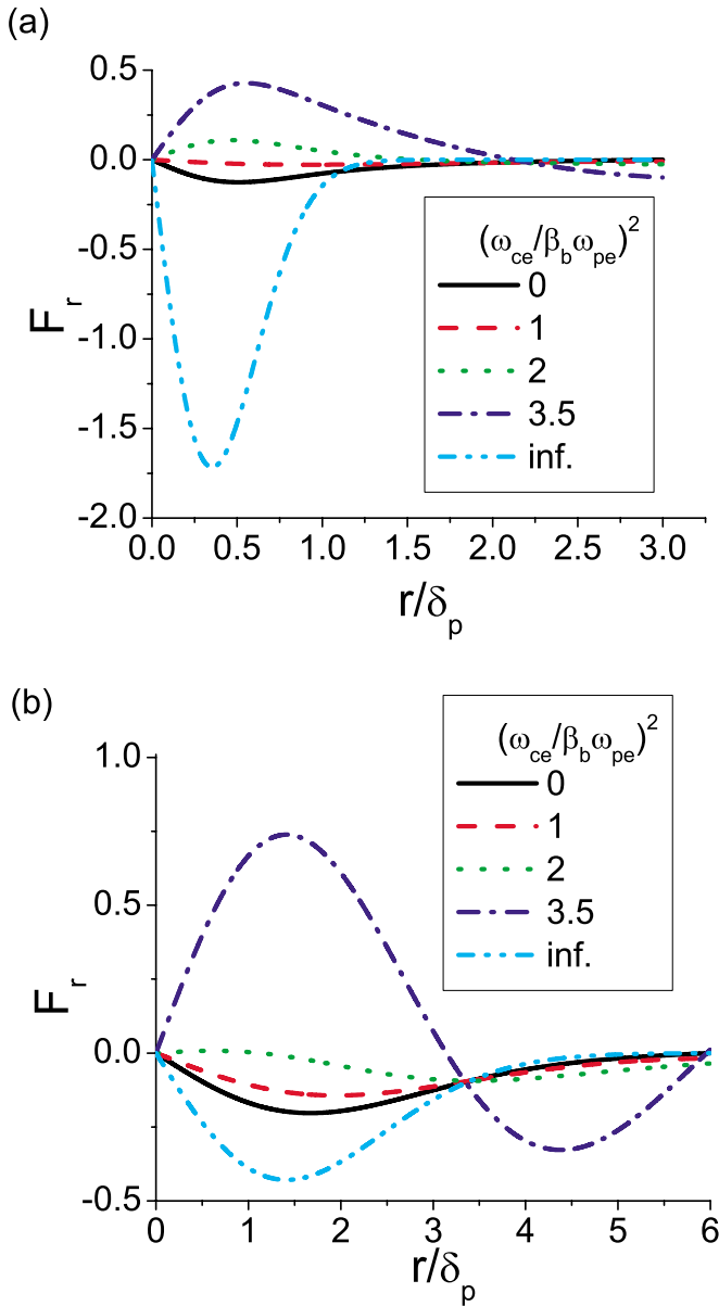
FIG. 14. (Color online) Plots of the normalized radial force acting on beam ions propagating through plasma for different values of (\omega_{ce}/\beta_b\omega_{pe})^2 calculated from Eqs. (23)–(27) for (\omega_{ce}/\beta_b\omega_{pe})^2 < 4 and Eq. (45) for (\omega_{ce}/\beta_b\omega_{pe})^2 \rightarrow \infty . The force is normalized to Z_b n_{b0} m V_b^2 \omega_{pe} / n_p c [see Eq. (36)]. The beam density profile is a Gaussian, n_{b0} \exp(-r^2/r_b^2) with (a) r_b = 0.5c/\omega_{pe} and (b) r_b = 2c/\omega_{pe} .
