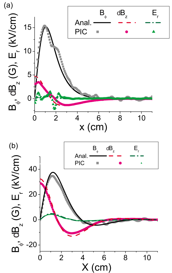
FIG. 11. (Color online) The azimuthal self-magnetic field, the self-magnetic field perturbation in the solenoidal magnetic field, and the radial electric field in a perpendicular slice of the beam pulse. The beam parameters are (a) n_{b0} = n_p/8 = 3 \times 10^{10} \text{ cm}^{-3} , V_b = 0.33c , and the beam density profile is taken to be Gaussian with r_b = 1 \text{ cm} . The applied magnetic field is (a) B_{z0} = 300 \text{ G} ; c\omega_{ce}/V_b = 0.57 , and (b) B_{z0} = 900 \text{ G} ; c\omega_{ce}/V_b = 1.7 .
