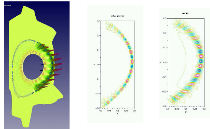
CMOD – n=20 eigenfunction. Pressure (l) and stream function (r)
