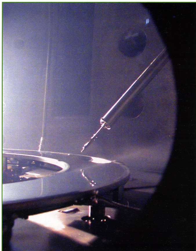
The pool of liquid lithium is shown in the toroidal tray that encircles the bottom of the CDX-U vacuum vessel. The tip of the liquid-lithium injector, which is removed before plasma operations, is reflected on the shiny surface of the liquid lithium.
