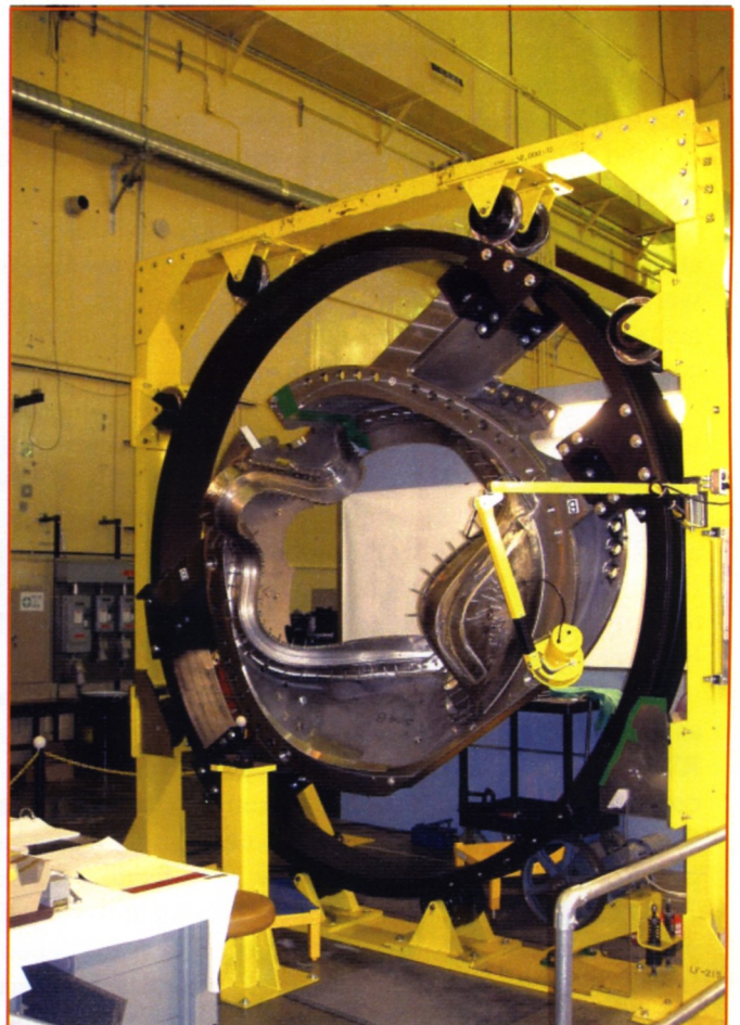
(Top, left) PPPL's Buddy Kearns and Mike Anderson prepare to lift the form out of the crate. (Top, right) Staff uncrate the form. (Bottom, left) PPPL's Mike Anderson installs modular coil parts on the winding form. (Bottom, right) The form after being mounted in PPPL's winding fixture.
