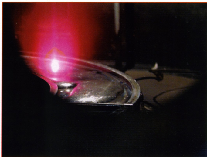
Above is an electron beam striking the lithium in the toroidal tray in CDX-U.
