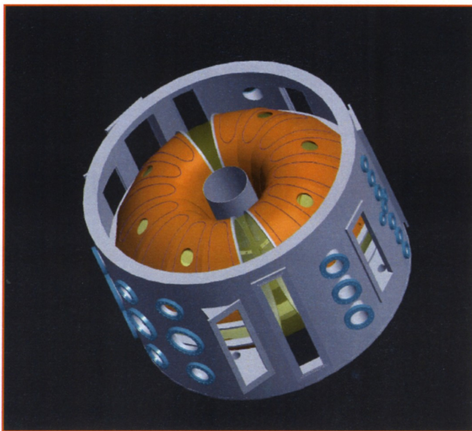
Above is a computer-generated drawing of the LTX shell inside the former CDX-U vacuum vessel.
