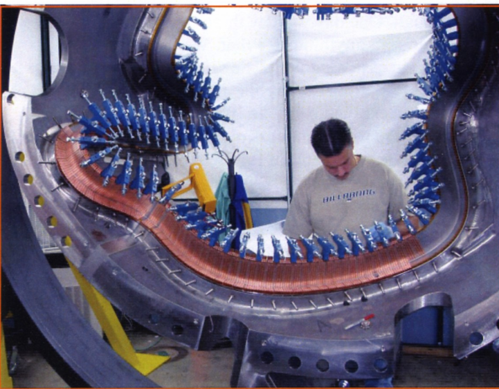
(Top, left) PPPL's Buddy Kearns and Mike Anderson prepare to lift the form out of the crate. (Top, right) Staff uncrate the form. (Bottom, left) PPPL's Mike Anderson installs modular coil parts on the winding form. (Bottom, right) The form after being mounted in PPPL's winding fixture.
