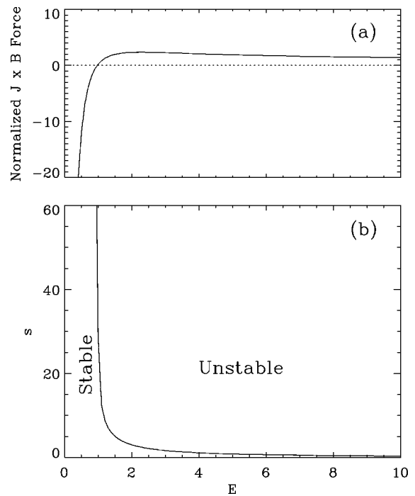
FIG. 11. (a) The \mathbf{j} \times \mathbf{B} force normalized by \xi_Z (B_0^2 / 2\mu_0) R_s as a function of E for a small axial shift. (b) The stability diagram for the axial shift mode in the parameter space of s and E with ion gyro-viscosity included.
