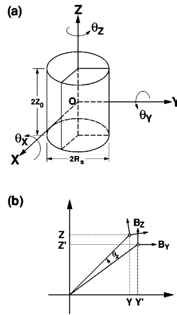
FIG. 2. (a) Three rotating axes (X,Y,Z) of the rigid body model. (b) Rotation of the vacuum field in the plasma frame.
