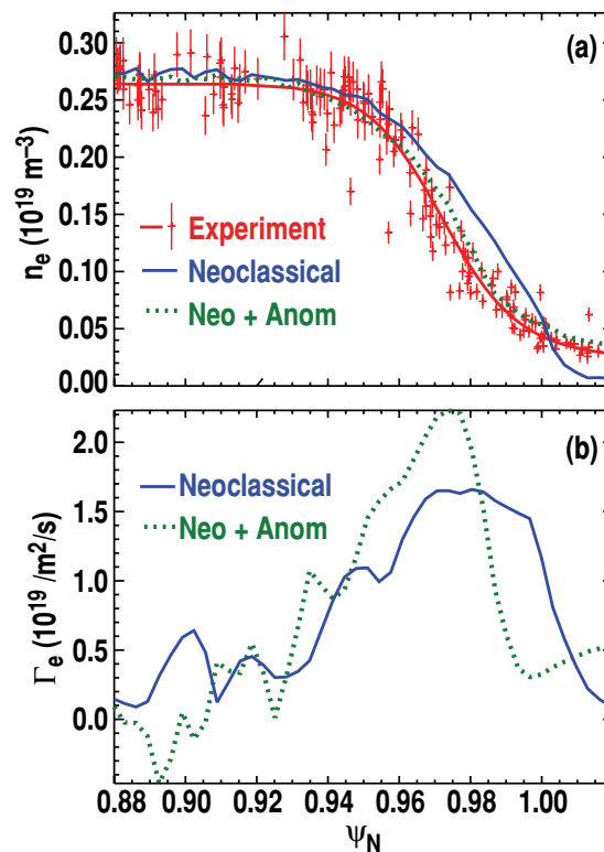
Figure 12. (a) Comparison of XGC0 model density profiles to the experimental density profile for DIII-D discharge 145716. Experimental n_e values (crosses), fit to experimental data (lighter solid line), modelled density profile with neoclassical transport (dark solid line), modelled density profile with neoclassical plus anomalous transport (dotted line). (b) Comparison of particle fluxes from the XGC0 neoclassical models with and without anomalous transport included.
