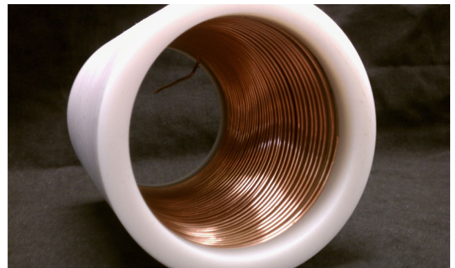
Fig. 5. A prototype ferroelectric plasma source with a white delrin outer jacket that holds the module assembly together axially and insulates the high voltage applied to the outer surface from the chamber wall. The inner electrode is made from a continuous helical copper winding to create better contact with the ceramic wall and provide increased electrode spacing.
