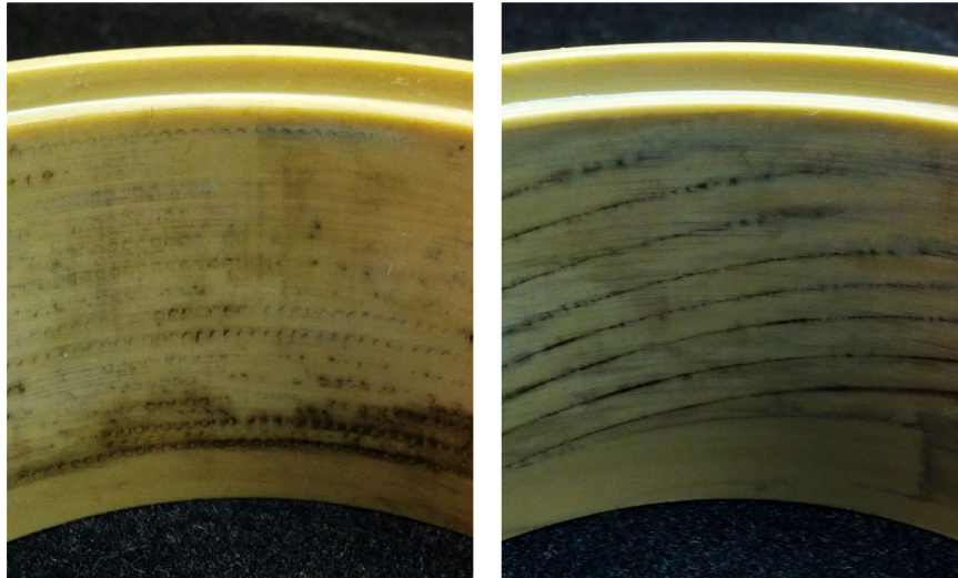
Fig. 6. (left) A faint regular square grid pattern is visible on the interior of a barium titanate ceramic ring after the perforated steel sheet electrode is removed. The black marks indicate the locations of plasma formation. (right) A clear series of black marks visible after the copper coil is removed show that the copper coil provides better contact, allowing for more uniform and dense plasma emission.
