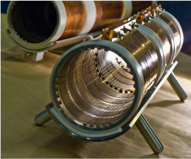
Fig. 3. The NDCX-II ferroelectric plasma source. The plasma source is assembled using 4.06 cm-long barium titanate rings that are stacked together to form modules of various lengths. Each ring is fitted with a rolled strip of perforated steel sheet that forms the inner electrode. Thin wires are drawn axially along the inner surface to ground the inner electrodes and to hold the module together. The high-voltage pulse is applied to the copper jacket that surrounds the exterior of the module.
