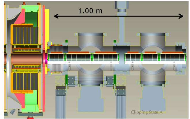
Fig. 4. A schematic of the proposed drift section of NDCX-II, in which the beam propagates from left to right, shows the final cell on the left with its stack of ferrite cores that drives the induction gap, and its pulsed solenoid for beam transport. The ferroelectric plasma source modules sit on aluminum cradles inside a bellows, two crosses, and a gate valve. To integrate properly with the system hardware, the plasma source modules shown here are constructed with three, five, five, three, three, and five rings.
