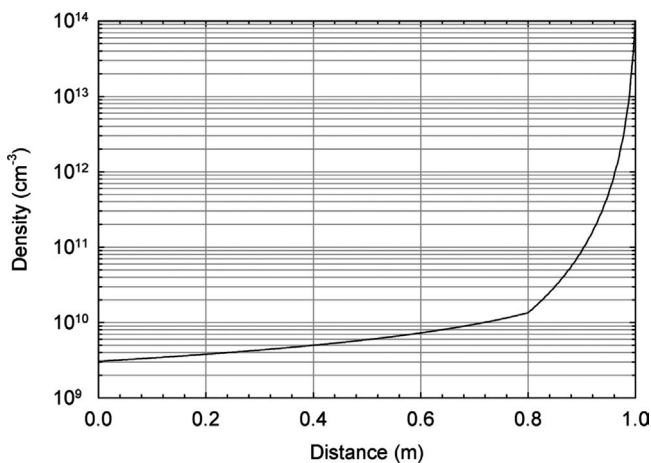
Fig. 1. The ion beam density plotted as a function of drift distance for a simple model in which the bunch length decreases linearly with distance and the radius is constant until 0.8 m, after which the radius decreases linearly with propagation distance. Here, a 50 nC charge bunch is assumed with a 2 cm initial radius and a 0.5 mm final radius.
