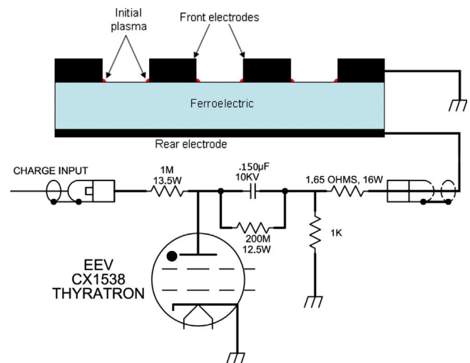
Fig. 2. A schematic drawing of the ferroelectric plasma source and its thyatron-switched pulser. The 150 nF storage capacitor is charged to high positive voltage, and when the thyatron switch is triggered, a large negative voltage appears on the rear electrode of the ferroelectric material.
