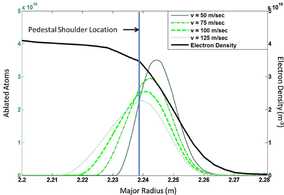
Fig. 9. Deposition of ablatant material for 600 \mu\text{m} granule at a range of injection velocities. The vertical blue line represents the shoulder of the pedestal. (For interpretation of the references to colour in this figure legend, the reader is referred to the web version of this article.)
