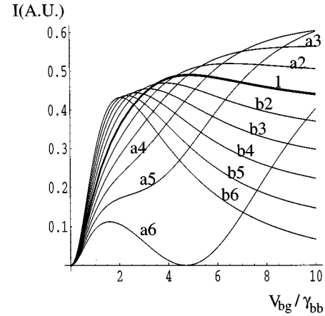
FIG. 7. Intensity of spontaneous emission vs V_{bg}/\gamma_{bb} for laser detuning \omega_{Lb}/\gamma_{bb} = -8 . Curves 1, a2..an..a6 correspond to successive values of q = 0.2(n-1) , curves b2..b6 are plotted for q = -0.2(n-1) with n = 2, \dots, 6 . Atomic parameters normalized to \gamma_{bb} are: \omega_{ab} = 10 , d_{bg}/d_{ag} = \sqrt{2} , \omega_{bg}/\omega_{ag} = 0.7 .
