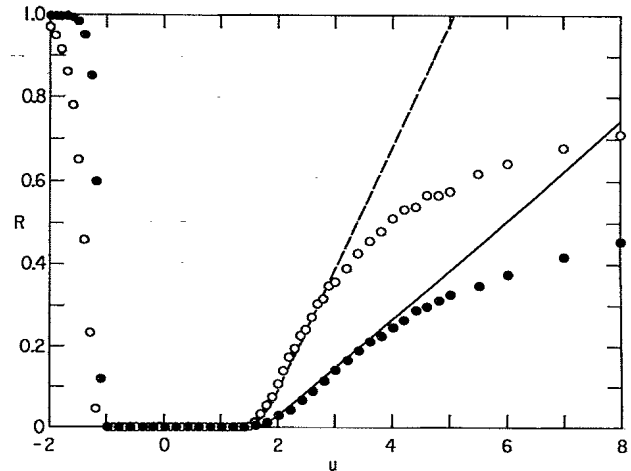
FIG. 2. The runaway fraction R(u, 1) vs u and R(u, -1) vs -u for Z=1 (closed circles) and Z=5 (open circles). The points show the results of the Monte Carlo method, the curves show approximate analytic fits near the "turn-on" region \mu=1 , u \geq 1 . For u > b , the form of the curves is R = a[(u-b)^4 - c^4] - ac ; for u \leq b , R=0 . For Z=1 , we have a=0.12 , b=1.4 , c=0.4 . For Z=5 , we have a=0.3 , b=1.3 , c=0.4 .
