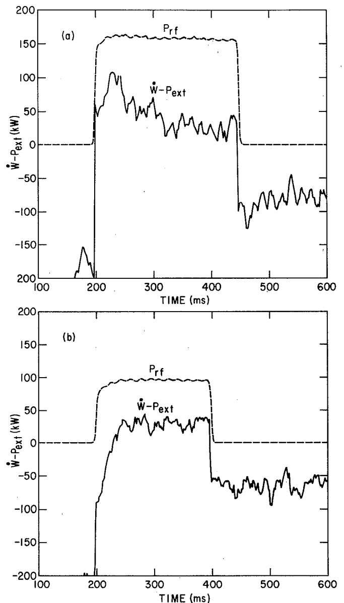
FIG. 2. Traces of \dot{W} - P_{ext} vs t for two representative ramp-up shots. In (a) P_{rf} = 160 kW and \dot{I} > 0 as soon as the rf is turned on. In (b) P_{rf} = 96 kW and there is a delay in \dot{I} changing sign.
