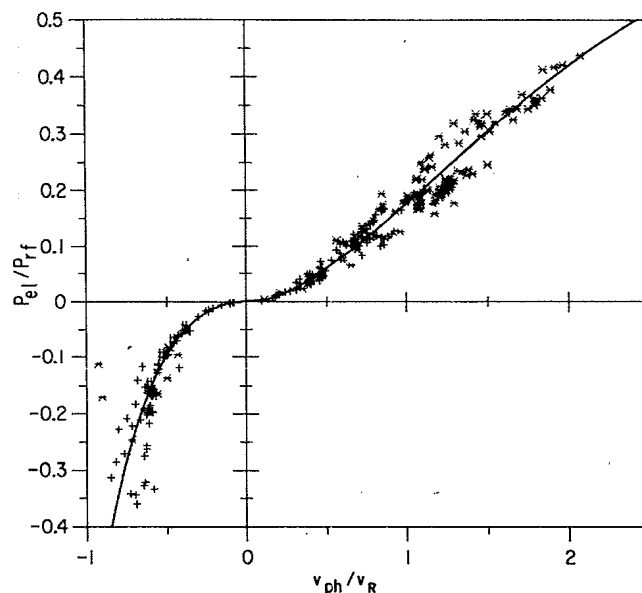
FIG. 1. P_{el}/P_{rf} vs u for 250 PLT shots. The rf power P_{rf} varied from 0 to 300 kW, the density n from 1.5 \times 10^{12} to 6.0 \times 10^{12} \text{ cm}^{-3} , the plasma current I from 150 to 400 kA. Three waveguide phasings were used 60^\circ (*), 90^\circ (+), and 135^\circ (#).
