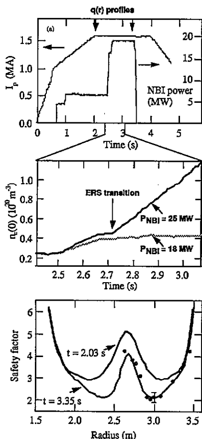
Figure 8. Time evolution (a) of the plasma current and NBI power for reversed shear scenario and expanded view, (b) showing central density and transition to R/S mode, and (c) the q profiles at two times.
