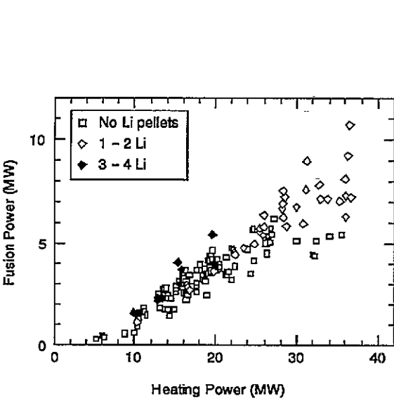
Figure 1. Dependence of peak DT fusion power on total heating power (NBI + ohmic).
