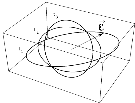
FIG. 2. Polarization of radiation when E_z \neq 0 .
