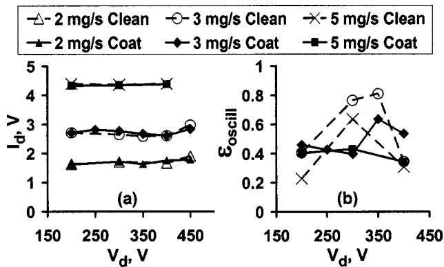
FIG. 1. Discharge current, I_d , and relative discharge current oscillations amplitude, \epsilon_{oscill} =amplitude/ I_d , vs discharge voltage, V_d , characteristics of the 123 mm HT. Measured at several mass flow rates for the clean and coated anodes.
