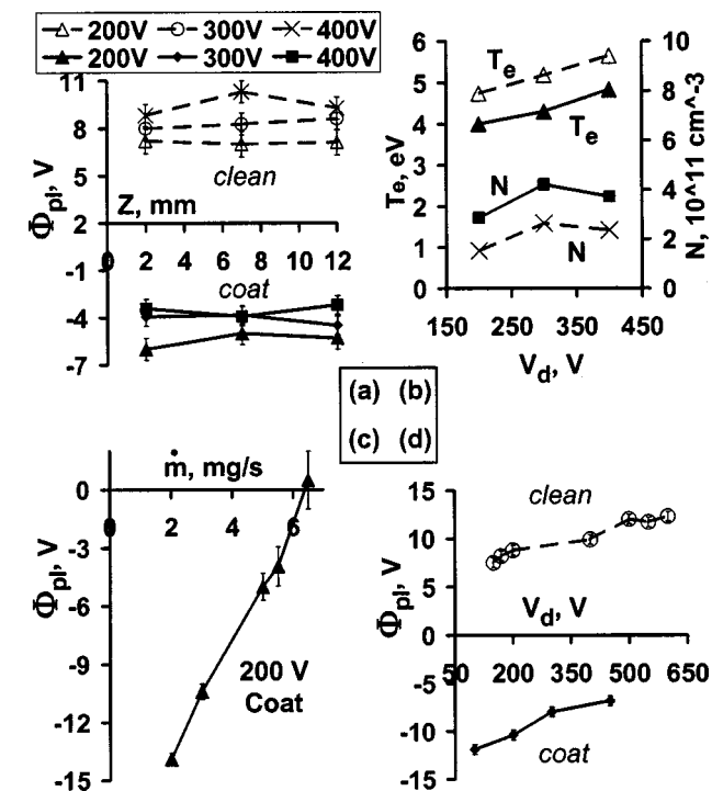
FIG. 2. Results of biased probe measurements in the near-anode region of the 123 mm HT. At the channel median: R=49 mm from the thruster axis. (a) Plasma potential axial profile, \Phi_{pl}(z) , for the clean and coated anodes measured at the mass flow rate \dot{m}=5 mg/s and several discharge voltages. Z=0 at the anode. (b) Electron temperature, T_e , and plasma density, N , vs discharge voltage, V_d , for \dot{m}=5 mg/s. At 7 mm from the anode. Open markers correspond to the clean anode, closed markers—to the coated anode. (c) \Phi_{pl} vs \dot{m} for the coated anode. At 7 mm from the anode. (d) \Phi_{pl} vs V_d for the clean and coated anodes. At 7 mm from the anode for \dot{m}=3 mg/s.
