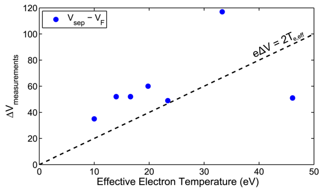
FIG. 14. (Color online) The difference between the separation point technique and the floating point technique versus temperature. Notice the large and varying differences between the two techniques.
