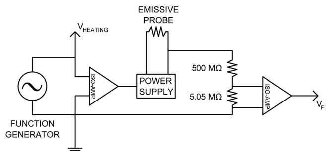
FIG. 5. The circuit diagram of the electronics used to measure the floating potential of an emissive probe at saturation.
