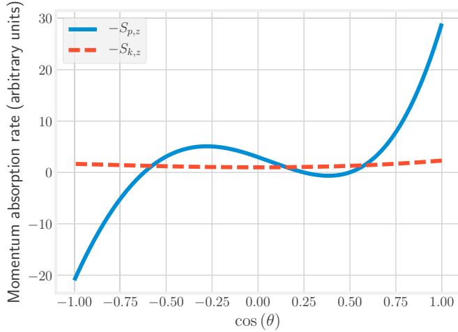
FIG. 3. The momentum absorption rate per electron as a function of \cos \theta = v_z/v for \beta = 0.08 : along the z axis taking into account the recoil (solid blue line), along the z -axis taking into account only the photon momentum (dashed red line).
