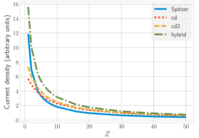
FIG. 4. The generated current density versus the ion charge Z : fluid approximation with the Spitzer conductivity given by Eq. (30) (solid blue line), current drive approximation keeping only the first term in Eq. (39) (dotted red line), current drive approximation keeping both terms in Eq. (39) (dashed orange line), hybrid current given by Eq. (41) (dash-dotted green line).
