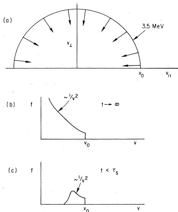
FIG. 45. Current drive exploiting a periodic inversion of the distribution of \alpha particles, which are born at 3.5 MeV (a) and tend towards a monotonically decreasing energy distribution (b). For short times, the \alpha particles temporarily assume an inverted energy distribution (c).
