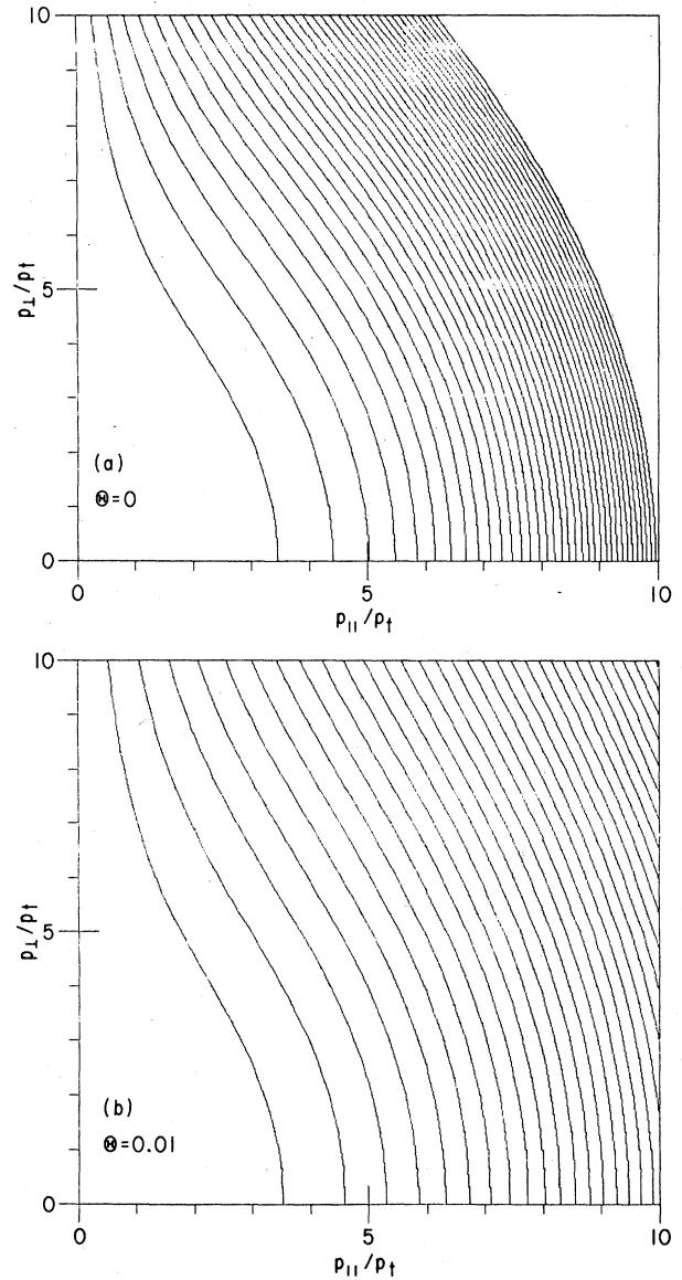
FIG. 18. Contour plots of \chi(\mathbf{p}) for Z=1 : (a) \theta=0 ; (b) \theta=0.01 . The contour levels are evenly spaced with increments of 50 \text{ } qp^4/m^2\Gamma . The higher levels are on the right-hand side, i.e., \partial\chi(\mathbf{p})/\partial p_{\parallel} > 0 (Karney and Fisch, 1986).
