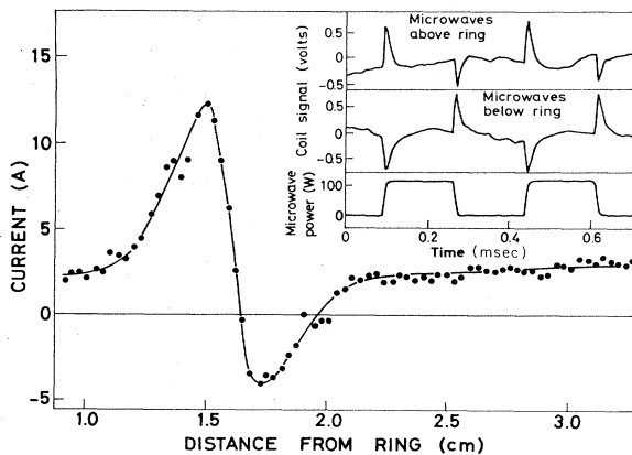
FIG. 42. Current vs probe position. Inset shows coil signals for rf input above and below the ring (Start et al. , 1982).
