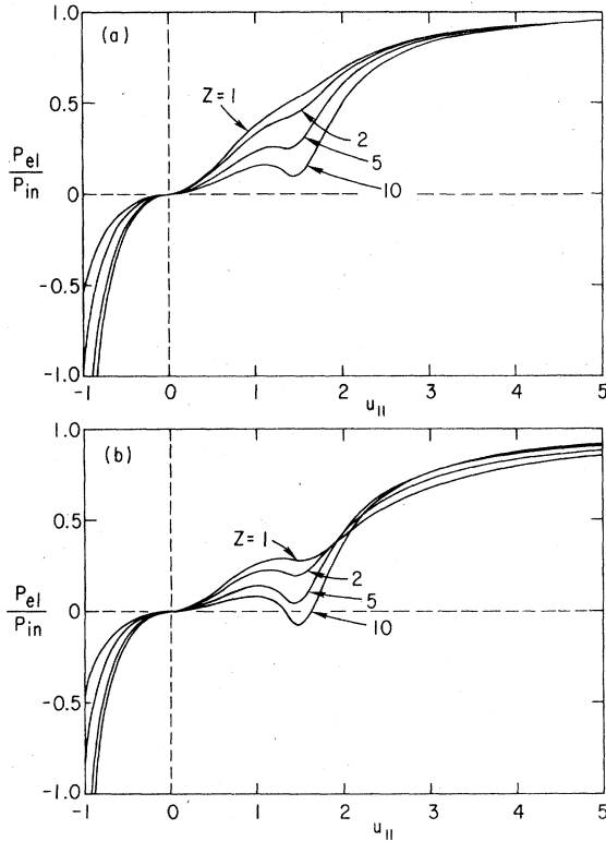
FIG. 17. Efficiency for two types of current drive: (a) lower-hybrid wave; (b) electron-cyclotron wave (Karney and Fisch, 1986).
