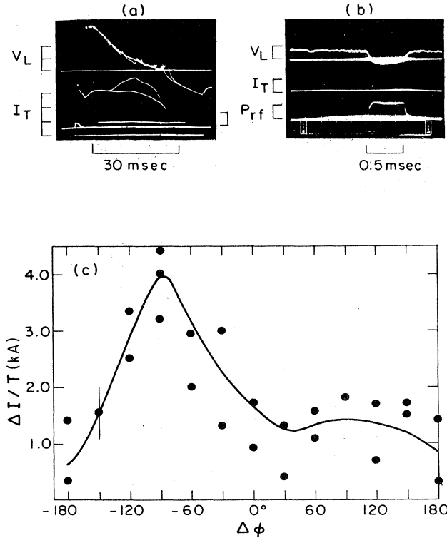
FIG. 35. Versator data. (a) Superimposed signals with and without rf power: one-turn loop voltage ( V_L ) 0.8 V/div; total current ( I_T ) 8 kA/div; rf power 30 kW/div. (b) Loop voltage with dI/dt=0 at high rf power: loop voltage 0.4 V/div; total current 4 kA/div (baseline suppressed); rf power 30 kW/div. (c) Current increment \Delta I_T normalized to rf power transmission coefficient T as a function of array; phase \Delta\phi with a 4-msec rf pulse. Plasma parameters, I_T=30 kA, n=2\times 10^{12} cm ^{-3} , B=8 kG (Luckhardt et al. , 1982).
