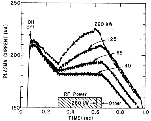
FIG. 37. Current vs time at n = 2.2 \times 10^{12} \text{ cm}^{-3} at different rf powers (Jobs et al. , 1985).
