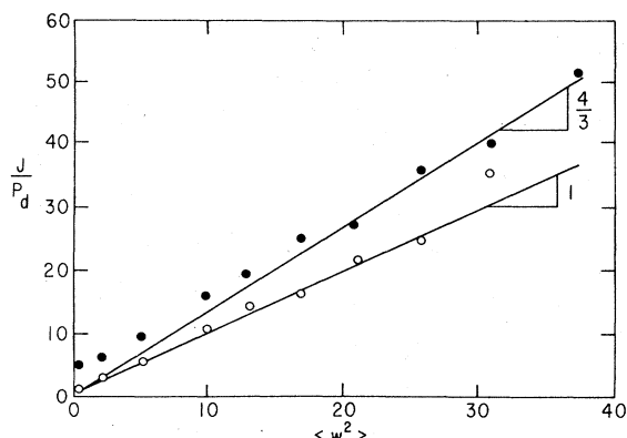
FIG. 9. Normalized efficiency J/P_d as a function of average w^2 in a narrow spectrum for small \mathbf{S}_w . The waves exist only for x < 1 . \circ , cyclotron damping; \bullet , Landau damping. Lines show the theoretical predictions of Eq. (2.25) (Karney and Fisch, 1981).
