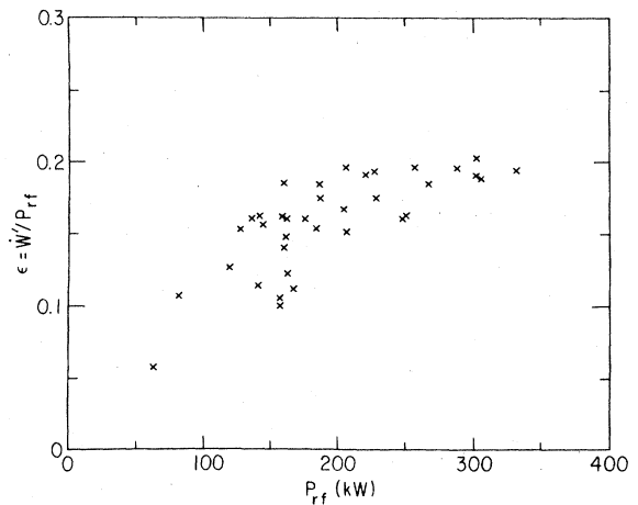
FIG. 38. Efficiency W'/P_{rf} vs injected rf power P_{rf} [where W' \equiv (d/dt)(LI^2/2) - P_{ext} ] for I = 200 \text{ kA} and a range of other parameters (Jobs et al. , 1985).
