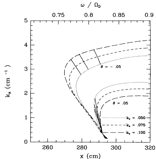
FIG. 1. Trajectory of IBW k_x(x) from dispersion relation of Eq. (7), with parameters: \omega = 1.69 \times 10^8 rad sec ^{-1} , n_e = 10^{14} cm ^{-3} , T_e = 10 keV, T_D = T_T = 20 keV, with fractional densities, f_D = f_T = 0.5 . The plasma inhomogeneity in the \hat{x} direction is due entirely to the variation in magnetic field \mathbf{B} = 4.8 \times 10^4(\hat{z} + \theta\hat{x})R/x G, with \theta = \pm 0.05 , and "major radius" R = 260 cm. The broken curves are trajectories for the values 0.05, 0.75, and 0.1 cm ^{-1} of the toroidal wave vector k_z . The solid lines connect the coordinates at which 0.75, 0.5, and 0.2 of the initial power remains.
