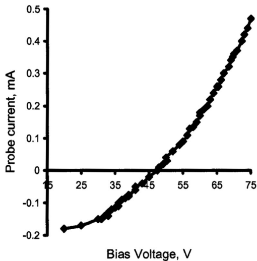
FIG. 3. Typical probe voltage–current characteristic (mass flow 1.7 g mg/s Xe, V_d=200 V, I_d=1.6 A, I_{\text{coil}}=1.5 A).
