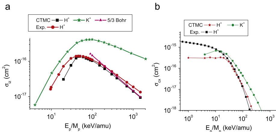
Fig. 9. Comparison of ionization cross-section (a), and (b) charge-exchange cross-sections for proton and potassium ion projectiles colliding with atomic hydrogen. The experimental data are from Refs. [1,3].
