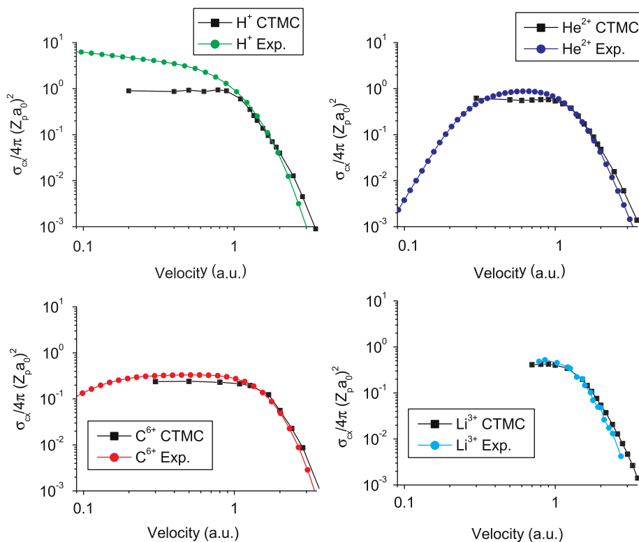
Fig. 4. Normalized charge-exchange cross-sections for collisions of fully stripped ions with atomic hydrogen. The experimental results are from Ref. [23] for H and He, Ref. [24] for Li, and Ref. [25] for C.
