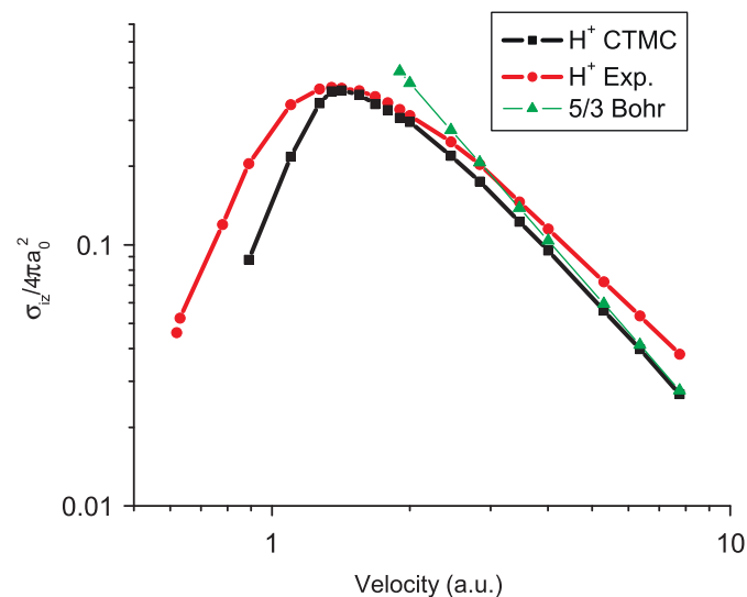
Fig. 2. Normalized ionization cross-section for proton collisions with atomic hydrogen in atomic units; the value of the cross-section is normalized to 4\pi a_0^2 = 3.517 \times 10^{-16} \text{ cm}^2 ; the velocity in atomic units can be calculated from the projectile energy per unit mass from v \text{ (a.u.)} = 0.2\sqrt{E \text{ keV/amu}} [1].
