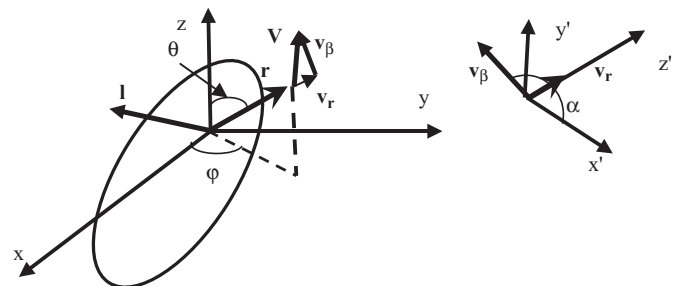
Fig. 1. Schematic of electron trajectory and definition of angles (\theta, \phi, \alpha) .
