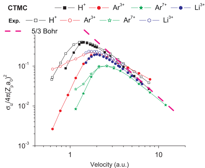
Fig. 5. Ionization cross-sections of argon ions ( \text{Ar}^{+3} and \text{Ar}^{+7} ) compared with fully stripped ions of the same charge ( \text{H}^+ and \text{Li}^{+3} ) on atomic hydrogen. The experimental values for Ar ions are taken from Ref. [26].
