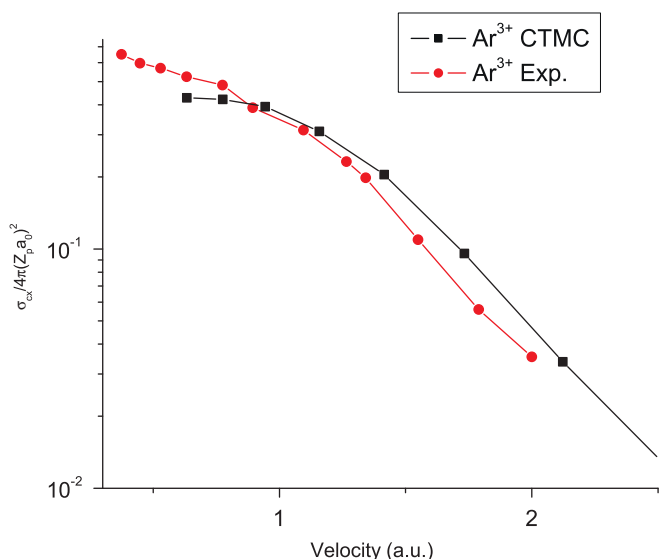
Fig. 6. Charge-exchange cross-sections for collisions of argon ions (Ar 3+ ) with atomic hydrogen. The experimental values were taken from Ref. [26].
