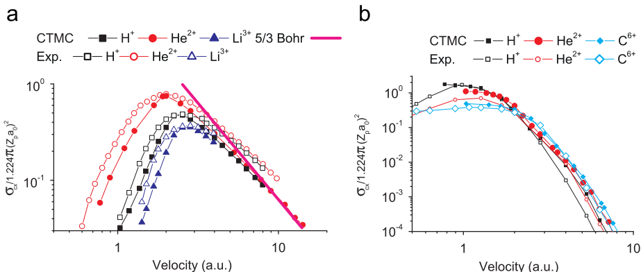
Fig. 7. Charge-changing cross-sections for fully stripped ions on helium corresponding to: (a) ionization, and (b) charge exchange. The experimental values were taken from [28]. The value of the cross-section is normalized to \pi a_0^2(Z_p E_0 / I_{nl})^2 = 1.224\pi Z_p^2 a_0^2 = 0.719 \times 10^{-16} Z_p^2 \text{ cm}^{-2} ; the projectile velocity in atomic units can be calculated from the projectile energy per unit mass from v \text{ (a.u.)} = 0.2\sqrt{E \text{ keV/amu}} [1].
