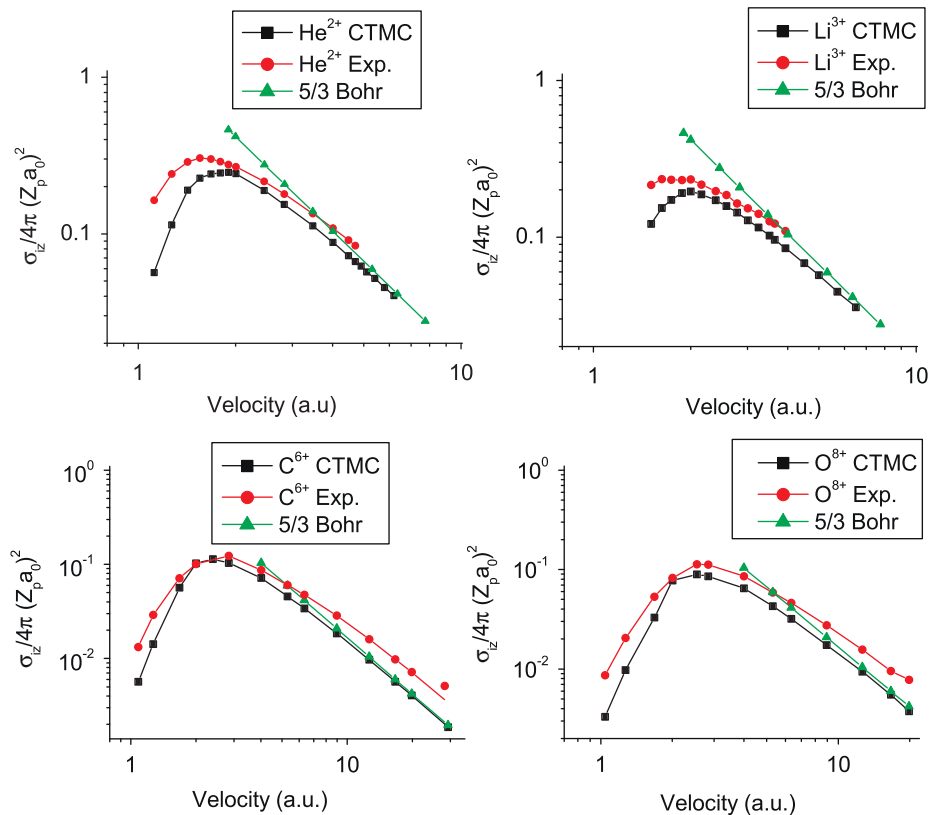
Fig. 3. Normalized ionization cross-sections for fully stripped ions colliding with atomic hydrogen; the value of the cross-section is normalized to 4\pi a_0^2 Z_p^2 = Z_p^2 3.517 \times 10^{-16} \text{cm}^2 . The experimental results for He, Li, and C and O are from Refs. [23,24] and [25], respectively.
