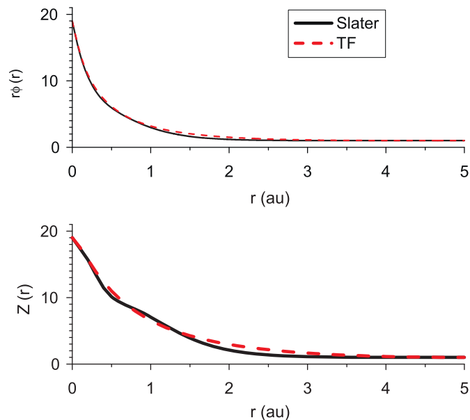
Fig. 10. Comparison of Thomas–Fermi and Slater models for the potassium ion potential, r\phi(r) , and profile of charge, Z(r) , inside a sphere of radius r . Note the differences between the two models at the outer edge of the ion. The orbital structure is evident for the Slater model.
