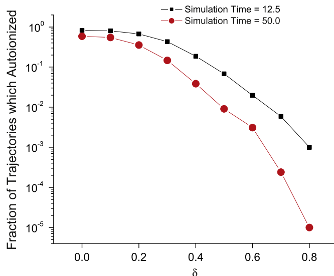
Fig. 11. Fraction of auto-ionizing two-electron helium atom orbits for two simulation time intervals.
