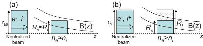
FIG. 8. (Color online) (a) Schematic illustration of a neutralized ion beam propagating along a strong solenoidal magnetic field with \Omega_e > \omega_{pe}^0 . The two possible regimes of collective beam focusing correspond to (a) quasineutral collective focusing, where quasineutrality is maintained inside the beam during compression, and (b) non-neutral collective focusing associated with a pronounced build-up of negative charge near the beam axis.
