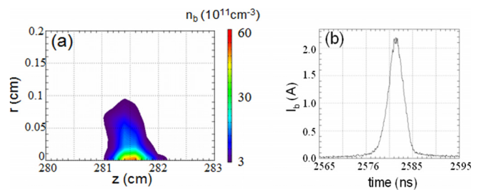
FIG. 6. (Color online) The ion beam parameters at the transverse focal plane. Shown are plots of (a) the ion beam density corresponding to t=2580 ns and (b) the time evolution of the ion beam current at the transverse focal plane corresponding to z=281.6 cm. The results are obtained using the LSP code.
