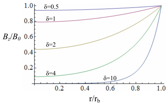
FIG. 14. (Color online) Radial dependence of the total magnetic field, i.e., the sum of the beam-induced and applied magnetic fields, for different values of \delta = r_b \omega_{pe}/c .
