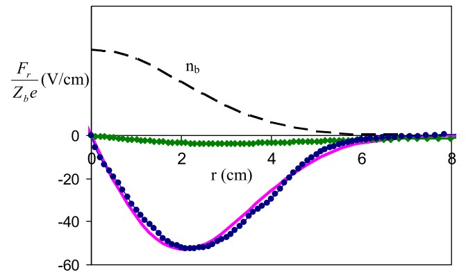
FIG. 3. Radial dependence of the normalized focusing force at the beam center. 14 The results of the numerical simulations correspond to B_0 = 300 G and \omega_{ce}/\beta_b\omega_{pe} = 18.7 (blue circles), and \omega_{ce} = 0 (green diamonds). The analytical results in Eq. (7) are shown by the solid pink curve. The beam parameters correspond to Z_b = 1 , r_b = 0.55 c/\omega_{pe} , l_b = 1.875 c/\omega_{pe} , \beta_b = 0.05 , and the plasma density is taken to be n_p = 10^{10} \text{ cm}^{-3} . The dashed black curve corresponds to the radial beam density profile, n_b = 0.14 n_p \exp[-r^2/r_b^2 - (z - V_b t)^2/l_b^2] . Results are obtained using the cylindrical (r, z) version of the LSP code. 25
