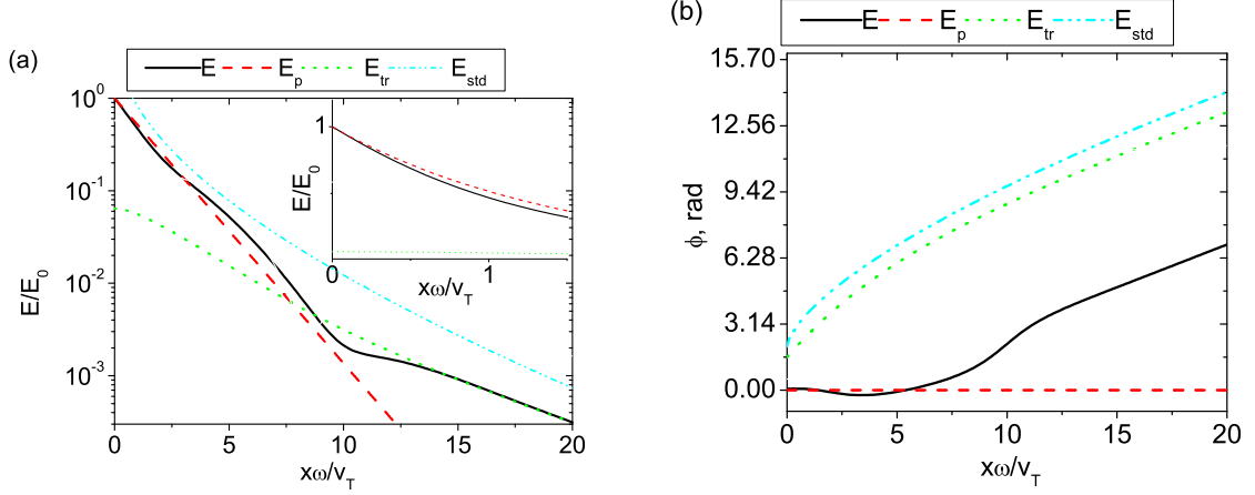
FIG. 11: Plot of the rf electric field as a function of the normalized coordinate x\omega/V_T for plasma parameters n = 10^{11}\text{cm}^{-3} , T_e = 3\text{eV} , f = 13.56\text{ MHz} (color online). Shown are (a) the amplitude and (b) the phase. Solid lines show the exact electric field profile E(x) calculated according to Eq. (60); dashed (red) line, the exponential part of the electric field E_p(x) = E_0 \exp(-k_p x) with k_p from Eq. (92); dotted line (green), the difference of the two E_t(x) ; and, chain (cyan) line, E_{std}(x) shows the asymptotic calculation for E_t in Eq. (C22). Subscript y is omitted in the electric field.
