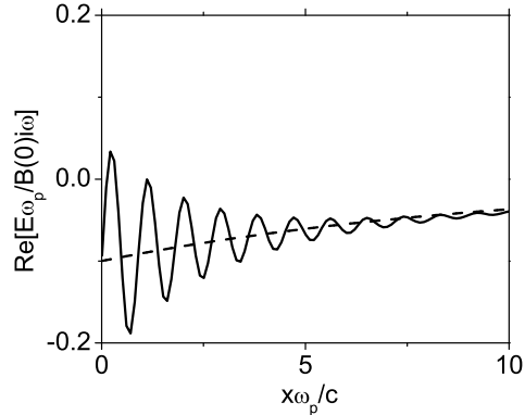
FIG. 14: The electric field in the plasma with v_{Ty} = 0.1c , \omega = 0.01\omega_p , T_y/T_x = 50 . The solid line shows the real part of the electric field profile obtained from the full solution. The dashed line corresponds to the smooth part of the solution \sim \exp(-\omega x/v_{Ty}) .
