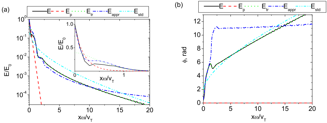
FIG. 12: Plot of the rf electric field as a function of the normalized coordinate x\omega/V_T for plasma parameters n = 10^{11}\text{cm}^{-3} , T_e = 3\text{ eV} , f = 1\text{ MHz} , similar to Figs. 9 and 10. Shown are (a) amplitude and (b) phase. Solid lines show the exact electric field profile E(x) calculated according to Eq. (60); dashed (red) line, the exponential part of the electric field E_p(x) = E_0 \exp(-k_p x) with k_p from Eq. (92); dotted line (green) the difference of the two E_t(x) ; chain (blue) line represents the limiting case of strong anomalous skin effect \Lambda \rightarrow \infty E_{appr}(x) , and dashed and double dotted (cyan) line shows E_{std}(x) , the asymptotic calculation for E_t in Eq. (C22). Subscript y for the electric fields is omitted.
