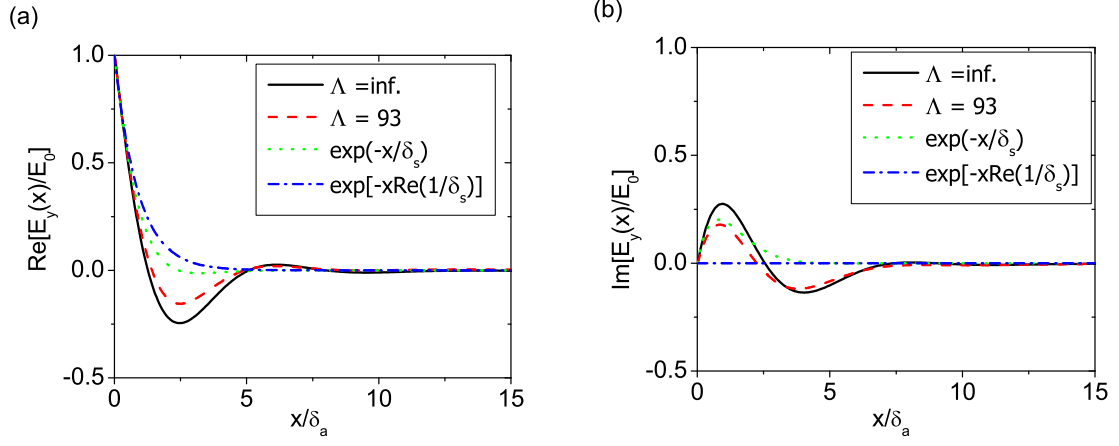
FIG. 9: Plot of the rf electric field as a function of the normalized coordinate x/\delta_a (color online). The solid (black) curve corresponds to the solution in the limit \Lambda = v_T\omega_p/c\omega = \infty ; dashed (red) line - \Lambda = 93 (plasma parameters n = 10^{11}\text{cm}^{-3} , T_e = 3\text{ eV} , f = 1\text{ MHz} ). The dotted (green) and dash-dotted (blue) lines shows the skin approximation in Eqs. (68) and (69): (a) real, and (b) imaginary part of the electric field.
