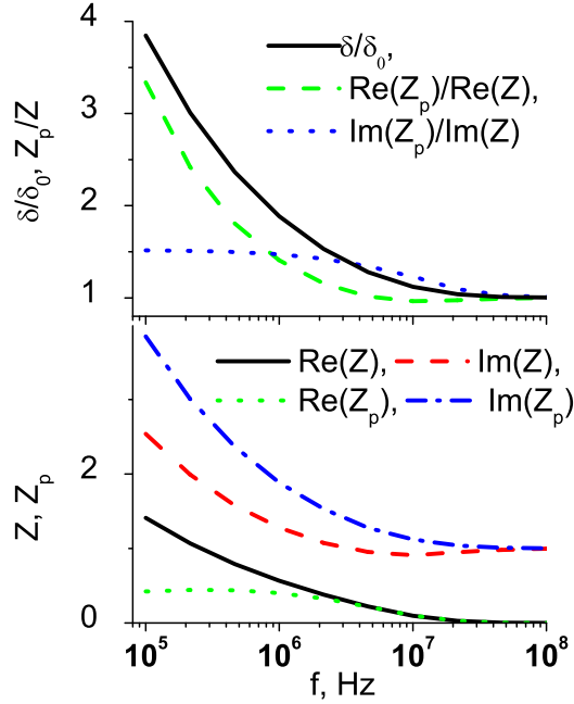
FIG. 13: Plot of the real and imaginary parts of the surface impedance versus discharge frequency calculated exactly making use of Eq. (100) and approximately using Eqs. (101) and (103) in the limit of collisionless plasma \nu \ll \omega (color online). Also shown is the ratio of the actual skin depth \delta = 1/k_p given by Eq. (92) to the skin depth calculated in the cold plasma approximation \delta_0 Eq. (49), (top).
