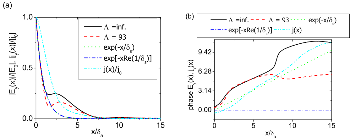
FIG. 10: Plot of the rf electric field and electron current as a function of the normalized coordinate x/\delta_a (color online). The same profiles as in Fig. 9, shown are (a) amplitude, and (b) phase with respect to the phase of the electric field generated by the field in vacuum.
