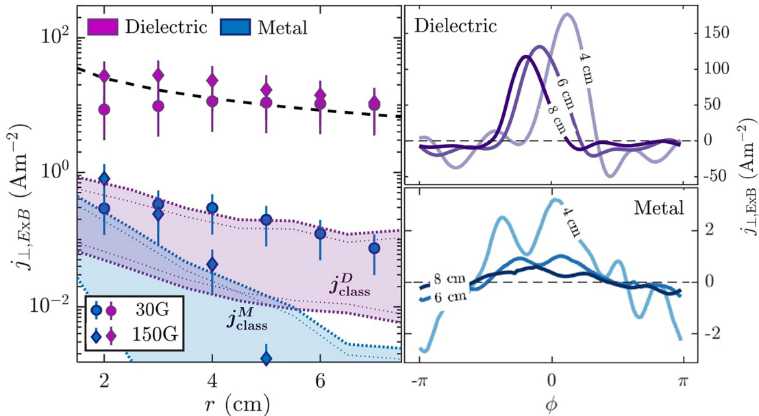
FIG. 5. (Left) Comparison of time averaged cross field anomalous current density with the radius for metal and glass boundaries, shown for B = 30, 150 G. The shaded regions represent classical transport estimates given measured gradients for values of B spanning 30–150 G. The broken black curve corresponds to a uniform distribution of I_d , i.e., j = I_d/2\pi r . (Right) Spoke phase resolved transport at different radii ( r = 4, 6, 8 cm), with \phi = 0 corresponding to the density maximum ( B = 30 G).
