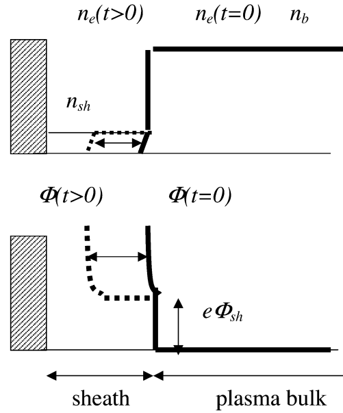
Fig. 5. Schematic of a sheath. Negatively charged electrode pushes electrons away at different distances depending on the strength of the electric field at the electrode. Shown are the density and potential profiles at two different times. Solid line is at the time of maximum sheath expansion.
