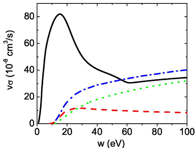
FIG. 6. (Color online) The frequency scaling of the electron impact collisions in xenon. (Solid black line) the elastic scattering; (dashed red line) excitation; (dotted green line) ionization; (dot-dashed line) the sum of ionization and excitation cross sections.
