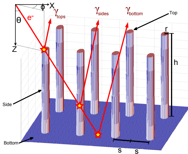
FIG. 1. Schematics of the velvet surface: the whisker geometrical quantities radius, r , height, h , and spacing, 2s . Also shown are electron velocity polar angle \theta , and velocity azimuthal angle, \phi . Numerical calculations include three contributions to secondary electron emission from velvet: electrons emitted by the side, top, and bottom surface of the whiskers.
