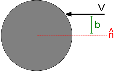
FIG. 6. Definition of the impact parameter, b . Cylinder is seen from tops, view aligned along z axis.
