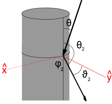
FIG. 5. Angle \theta is the polar angle of the primary electron. Angle \theta_2 is the polar angle of the secondary electron. Angle \vartheta_2 is the local normal angle of the secondary electron. \phi is the primary azimuthal angle. \phi_2 is the secondary azimuthal angle.
