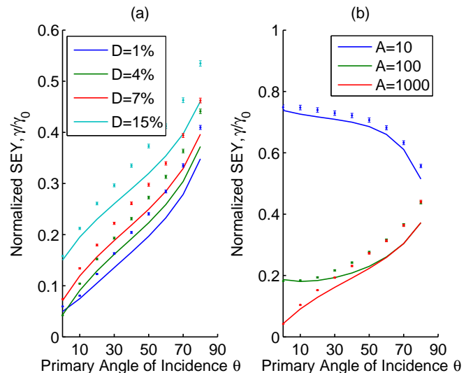
FIG. 3. SEY reduction from the case of normal incidence on a flat surface. SEY reduction is given as a function of incident angle, \theta , for different values of whisker aspect ratio A , and packing density D . Figure (a) shows SEY for 4 different D values and the same A = 1000 . Figure (b) shows SEY for 3 different values of A and the same D = 4\% . Solid lines show the result of an analytic approximation. Points with error bars are the result of these Monte Carlo simulations. The simulation results are compared to the analytic approximation given in section IV, Eq.23.
