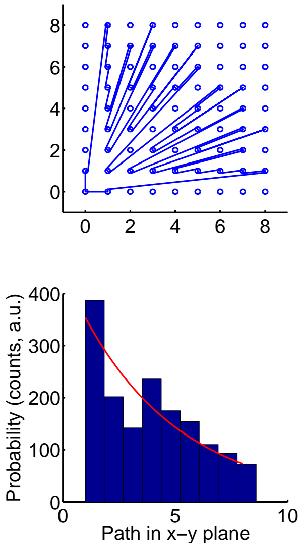
FIG. 4. Top: Schematics showing the top view of the velvet with regular pattern of whiskers for D = 4\% . Blue lines show the maximum extent of trajectories emitted at 1500 values of \phi , evenly spaced between 0 and \pi/2 , originating at point 0,0. Bottom: Probability histogram of mean-free-path for D = 4\% for the rectangular case. 1500 trajectories, evenly spaced in \phi , were calculated. The red curve is \exp(-l_{\perp}/\lambda_{\perp}) , corresponding to random configuration of whisker positions.
