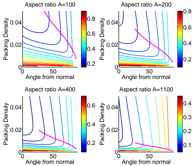
FIG. 8. Reduction of Secondary Electron Yield (ratio of the net SEY to that of a flat surface) as function of whiskers packing density and incident angle. Magenta line shows optimal value of packing density D(\theta) corresponding to the minimum net SEY.
