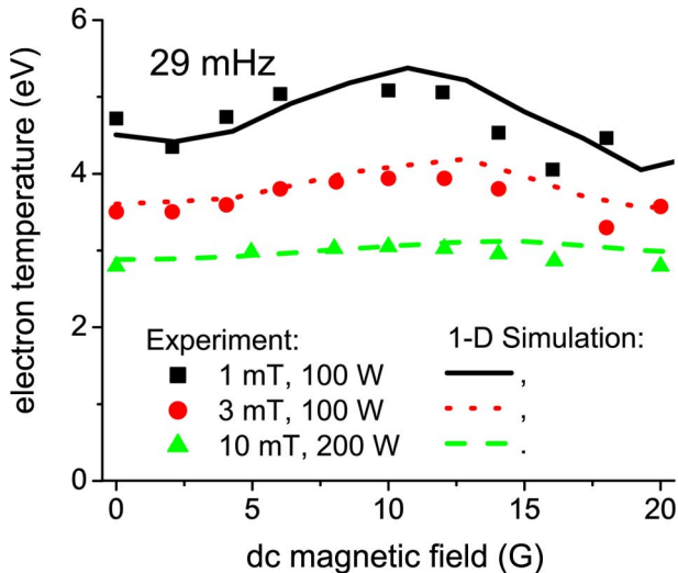
Fig. 22. Electron temperature at the discharge center as a function of the applied magnetic field for full self-consistent discharge simulations for different deposited powers and gas pressures. Case of one grounded electrode. Discharge parameters are the same as in Fig. 19. (Color version available online at http://ieeexplore.ieee.org .)
