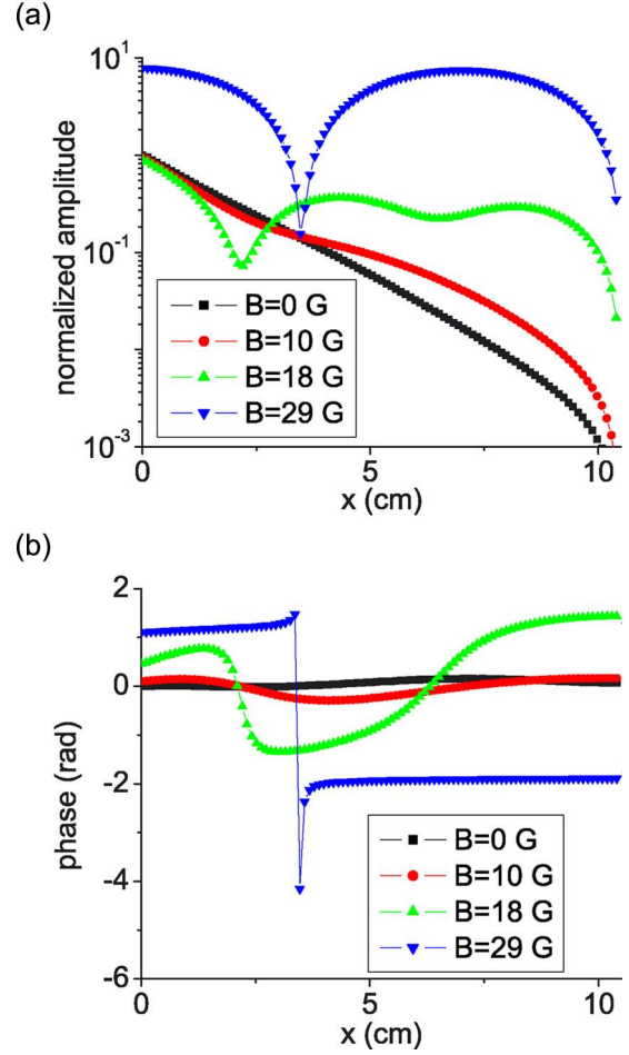
Fig. 14. Electric field profiles normalized by the electric field E(x=0, B=0) : (a) amplitude and (b) phase for different values of applied magnetic field for a uniform, bounded plasma. Plasma parameters are: half plasma length L/2 = 10.5 cm, RF field frequency \omega/2\pi = 29 MHz, electron temperature T_e = 4 eV, electron collision frequency \nu = 1.2 \cdot 10^7 s ^{-1} , and the plasma density n_e = 10^{11} cm ^{-3} [33]. (Color version available online at http://ieeexplore.ieee.org .)
