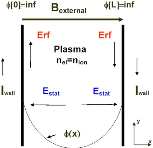
Fig. 13. 1-D model of magnetized ICP. The external magnetic field goes perpendicularly to walls. RF electric field has also a component along z axis. (Color version available online at http://ieeexplore.ieee.org .)
