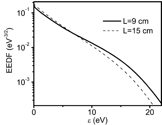
Fig. 7. EEDFs for the bounce resonance discharge gap length, L = 9 cm, and for nonresonant discharge gap L = 15 cm, for the surface current I = 1 A/cm, and other conditions are the same as in Fig. 7.
