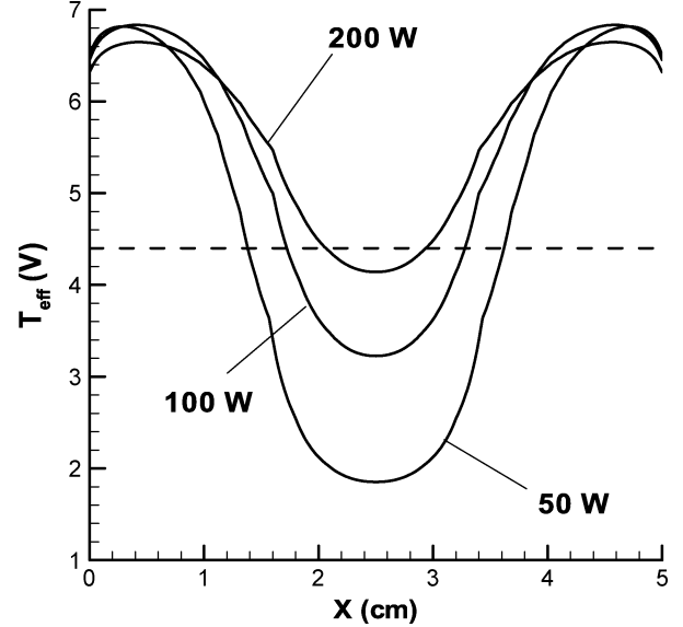
Fig. 9. Effective temperature profiles for a non-Maxwellian EEDF (solid lines) and a Maxwellian EEDF (dashed lines) for 1 mtorr [30], [40].
