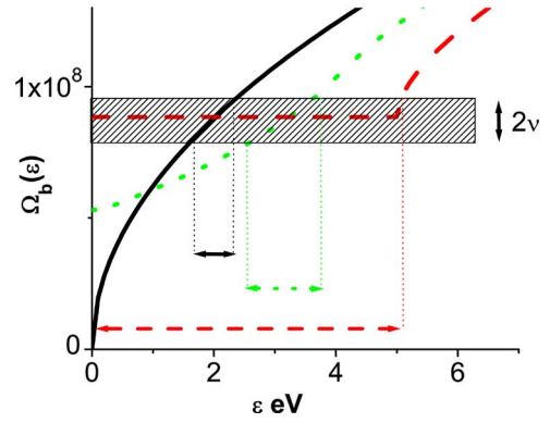
Fig. 2. Electron bounce frequency \Omega_b(\varepsilon_x) , as a function of the electron energy \varepsilon_x = mv_x^2/2 - e\phi(x) for different potential wells, consisting of the reflecting walls and different ambipolar potentials \phi(x) . Solid line corresponds to a uniform plasma with \phi(x) = 0 , dashed line quadratic potential \phi(x) = 5 \times (2x/L - 1)^2 eV and dotted line; the realistic potential obtained from the ion fluid model with T_e = 5 eV. Discharge length is L = 3 cm. Box of height 2\nu shows the resonance region, corresponding to \omega = 8.52 \cdot 10^7 s ^{-1} . Arrows show electron energies in the resonance region [6]. (Color version available online at http://ieeexplore.ieee.org .)
