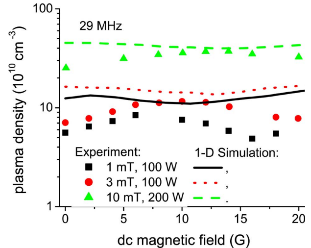
Fig. 23. Electron plasma density at the discharge center as a function of the applied magnetic field for full self-consistent discharge simulations for different deposited powers and gas pressures. Case of one grounded electrode. Discharge parameters are the same as in Fig. 19. (Color version available online at http://ieeexplore.ieee.org .)
