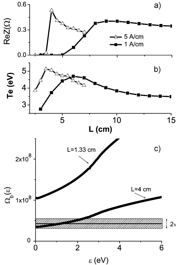
Fig. 6. Self-consistent simulations for coil currents I = 1 A/cm and I = 5 A/cm and the given discharge parameters: P = 3 mtorr, \omega/2\pi = 6.78 MHz. Shown are: (a) the plasma surface resistance; (b) the electron temperature in the discharge center versus the discharge gap; and (c) the electron bounce frequency [6].
