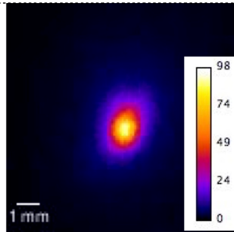
Figure 1. The transverse ( x , y ) distribution of the \text{He}^+ beam is shown with a color calibration bar indicating the relative intensity. With the new helium source, NDCX-II can provide 1-MeV helium ion beams with an energy deposition greater than 0.7 joules/cm 2 ( \sim 40 A/cm 2 ).
