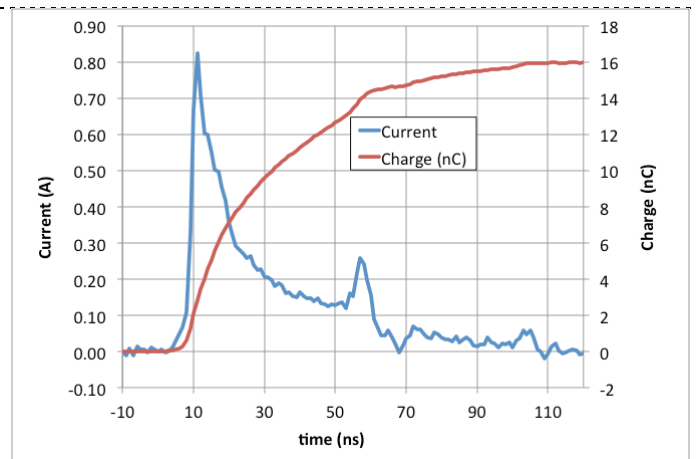
Figure 2. The full temporal distribution of the pulses is \sim 50 ns with a \sim 1 ns rise time, though still with a broader tail than desired. The integrated charge in the pulse is \approx 15 nC. The pulse was measured with a fast Faraday collector isolated from the neutralizing plasma with hole plates with low geometric transparency.
